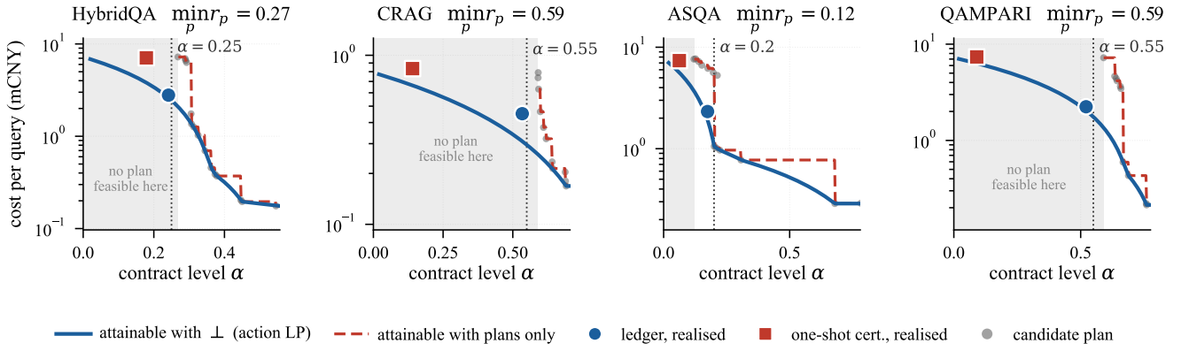
Figure 2: Cheapest attainable cost as a function of the contract level. Small dots are the individual plans; the dashed staircase is the cheapest of them that clears \alpha , which is what a system obliged to answer every query can reach, and it stops at the risk floor \min_p r_p . The solid curve adds the decline action, is continuous, and extends into the shaded region where no plan is feasible. Large markers are where each method operates at the median contract level, plotted at its realised risk: both mix a plan with \perp , so both can sit left of the floor, but the ledger sits close to the attainable curve while the certificate sits well above and to the left of it. That displacement is unspent allowance, and it is paid for in money.
