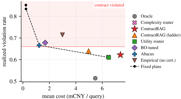
QAMPARI (citation), \alpha = 0.66
