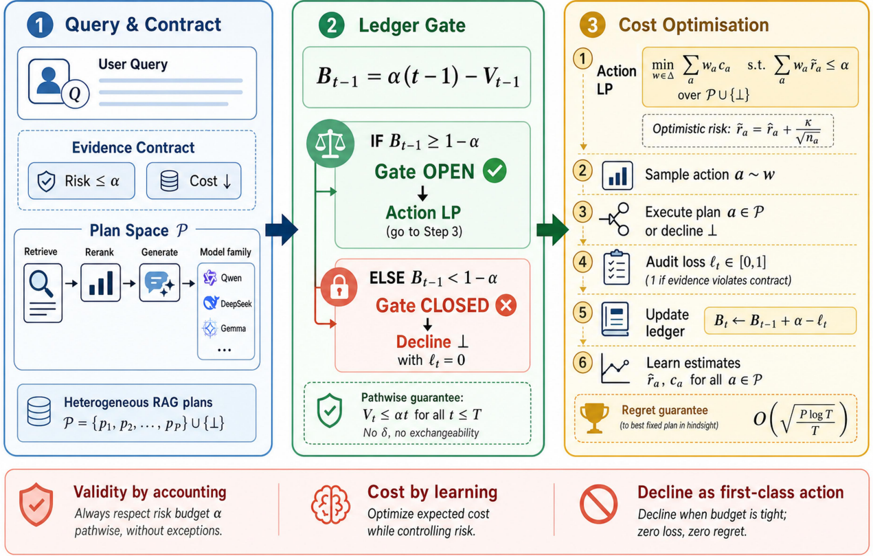
Figure 2: Overview of ledger-gated execution. A query arrives under an evidence contract and a heterogeneous plan space that includes the decline action \perp (left). The ledger gate opens only when the unspent allowance can absorb a worst-case loss, otherwise the arrival is declined at zero contract loss (centre). When the gate is open an optimistic action LP spends the allowance on cost, the chosen plan is executed and audited, and the ledger is updated (right). Validity is discharged by accounting; statistics serve cost alone.
