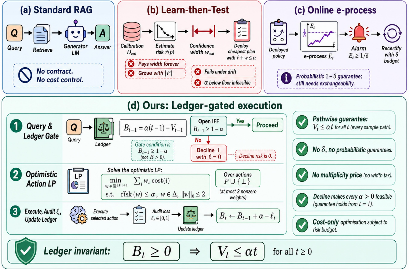
Figure 1: From statistical certification to accounting. (a) A plain RAG pipeline carries no rate contract. (b) Learn-then-Test certifies a plan on a calibration sample and pays a confidence width forever; the width grows with |P| and any level below the risk floor is infeasible. (c) An online e-process can raise an alarm and trigger recertification, but the guarantee remains probabilistic and assumption dependent. (d) Ledger-gated execution replaces the certificate with a deterministic gate B_{t-1} \geq 1 - \alpha , an optimistic action LP over plans plus declining, and an audited ledger update; validity is an identity of the trajectory and cost is a pure learning problem.
