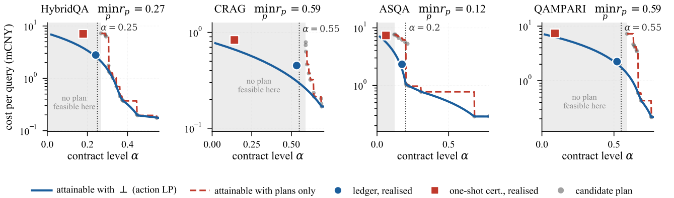
Figure 6: Cheapest attainable cost as a function of the contract level. Small dots are the individual plans; the dashed staircase is the cheapest of them that clears \alpha , which is what a system obliged to answer every query can reach, and it stops at the risk floor \min_p r_p . The solid curve adds the decline action, is continuous, and extends into the shaded region where no plan is feasible. Large markers are where each method operates at the median contract level, plotted at its realised risk: both mix a plan with \perp , so both can sit left of the floor, but the ledger sits close to the attainable curve while the certificate sits well above and to the left of it. That displacement is unspent allowance, and it is paid for in money.
