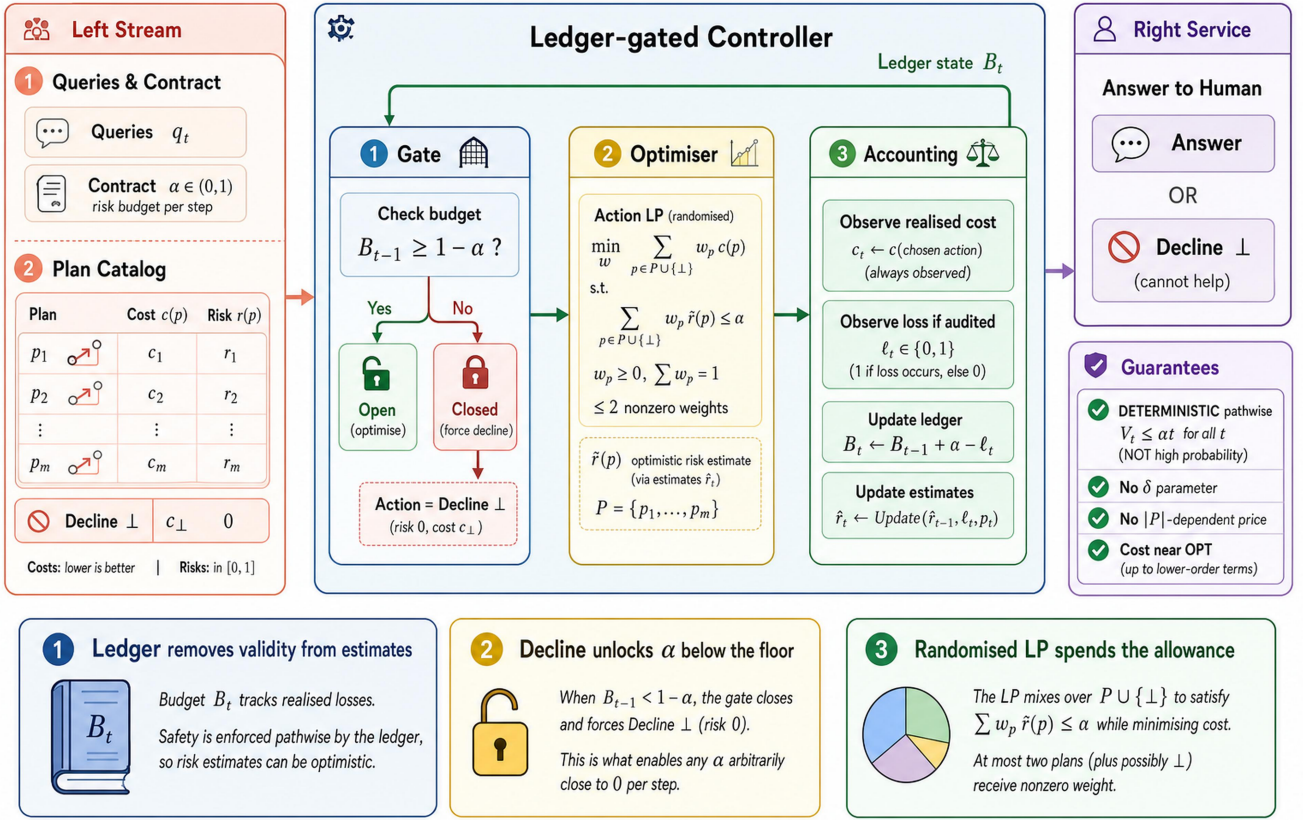
Figure 3: Per-arrival controller. The stream supplies the contract and the plan catalog (left). The gate, the optimistic action LP and the ledger update form a closed loop whose only feedback is the realised allowance B_t (centre). The service either answers or declines (right). The three ingredients at the bottom are individually useless: without the ledger the optimiser cannot be aggressive; without declining strict contracts are infeasible; without randomisation the controller cannot interpolate between plan risks.
