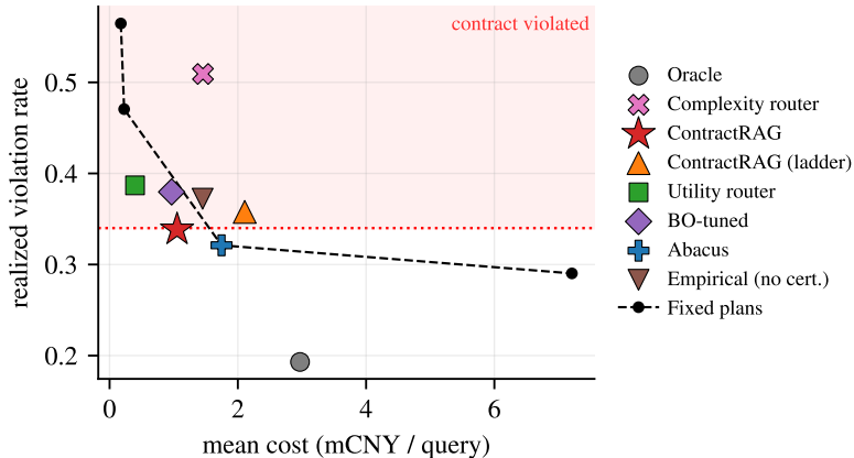
HybridQA (quality), \alpha = 0.34
