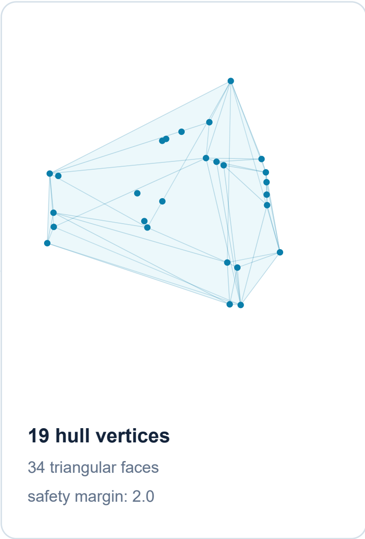
(b) Convex-hull space
