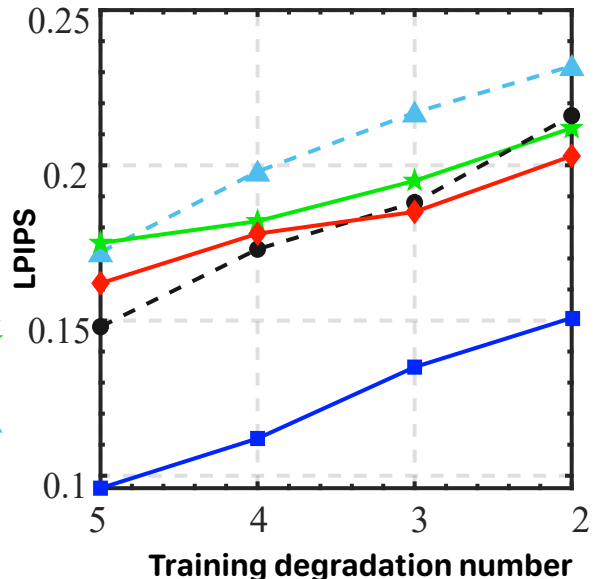
(b): Generalization results on JPEG artifact correction
