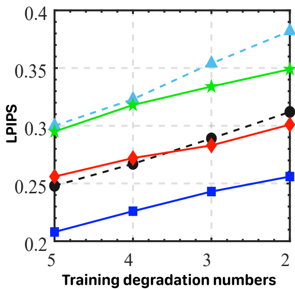
(a): Generalization results on underwater image enhancement
