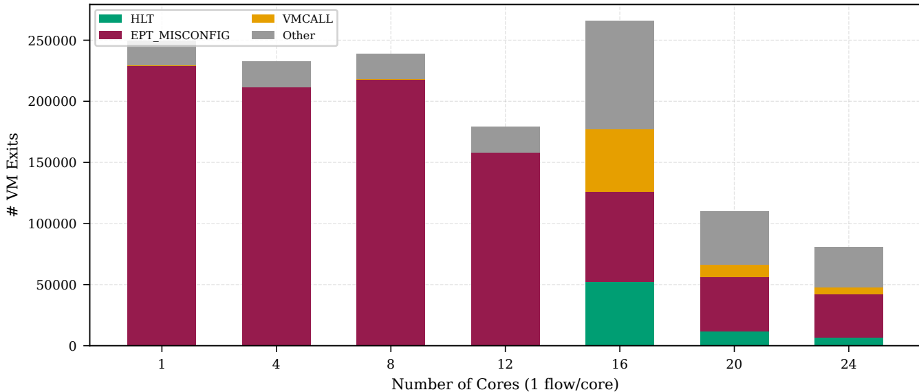
VM Exit Counts by Type
