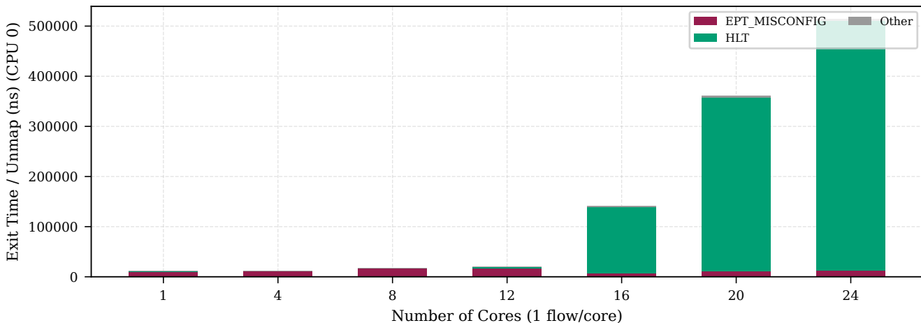
VM Exit Time per Unmap Call by Type
