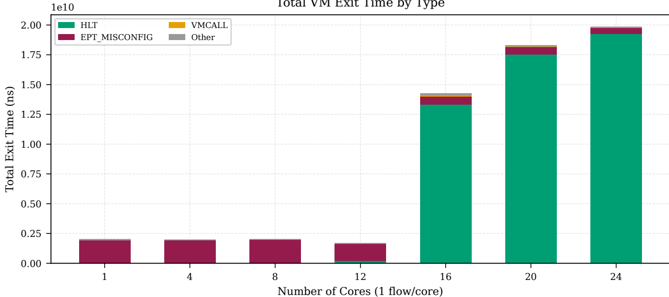
Total VM Exit Time by Type
