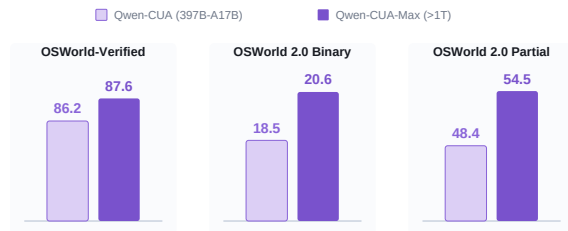
Figure 9: Scaling Qwen-CUA to Qwen-CUA-Max.
