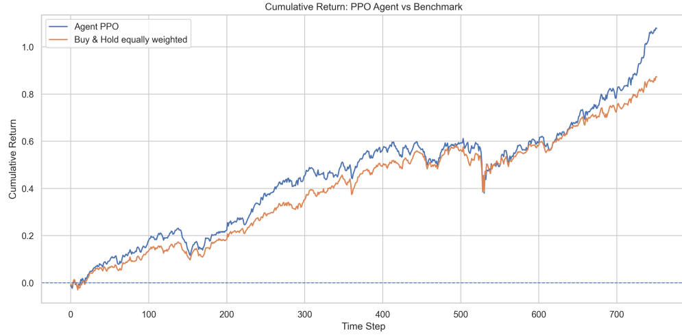
Figure 2: Cumulative return of the PPO agent compared with the buy-and-hold benchmark.
