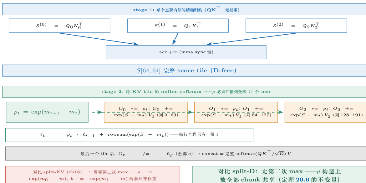
跨 chunk 两阶段合并 ( C = 3, D = 192 示例)
