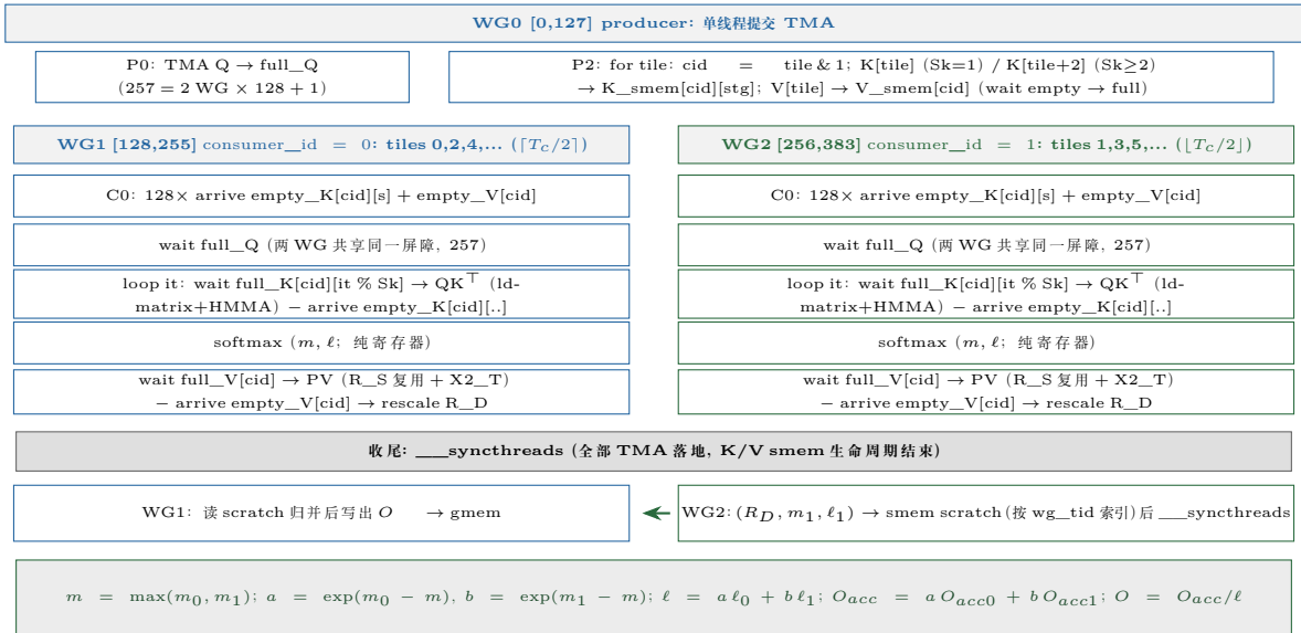
FA3 双 consumer 角色图 (384 线程, B_r = B_c = 64 )
