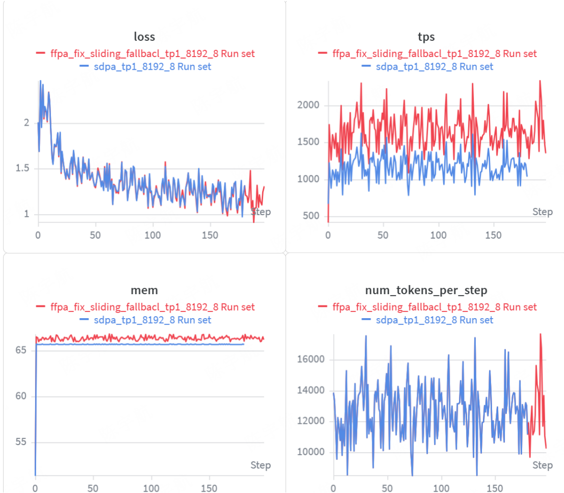
Figure 4: End-to-end training throughput on Gemma4-31B (8 \times H200, FSDP2, 8K sequence length). FFPA accelerates the 10 D=512 attention layers, achieving 1.4–1.5 \times overall throughput improvement at the same memory footprint as SDPA.
