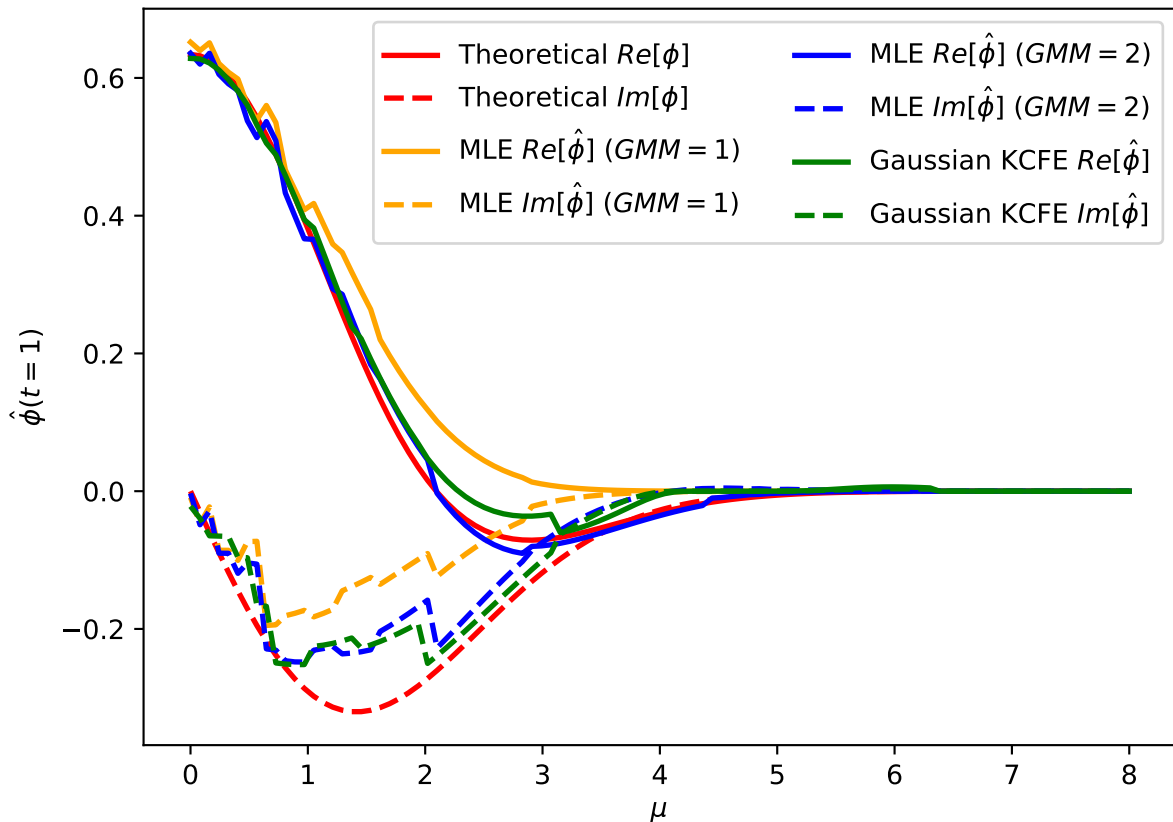
\phi(t=1) estimation with Gaussian noise inversion, \kappa = 0.9
