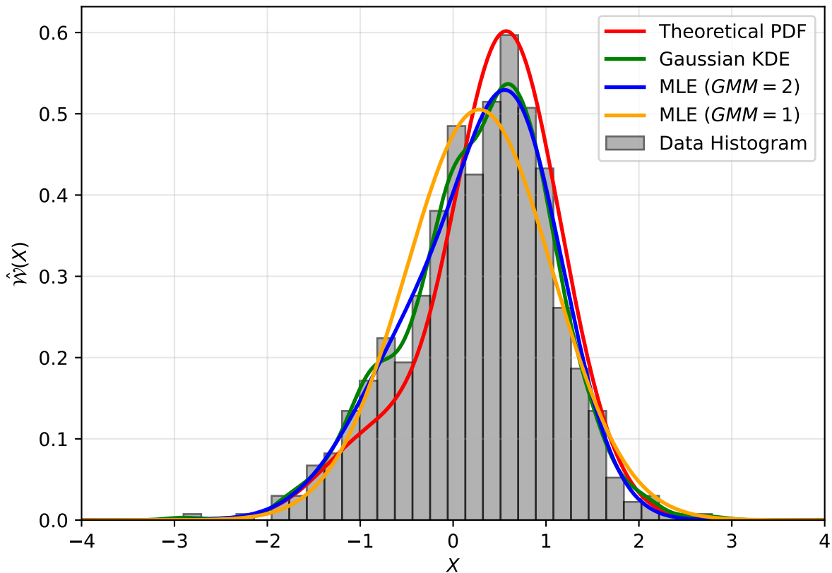
\hat{\mathcal{W}}(X) Estimation for n \approx 707 , \theta \approx 0.24
