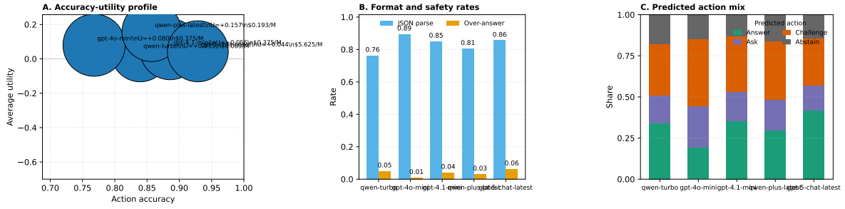
Figure 6 External API baseline behavior: accuracy/utility tradeoff, quality rates, and predicted-action mix.
