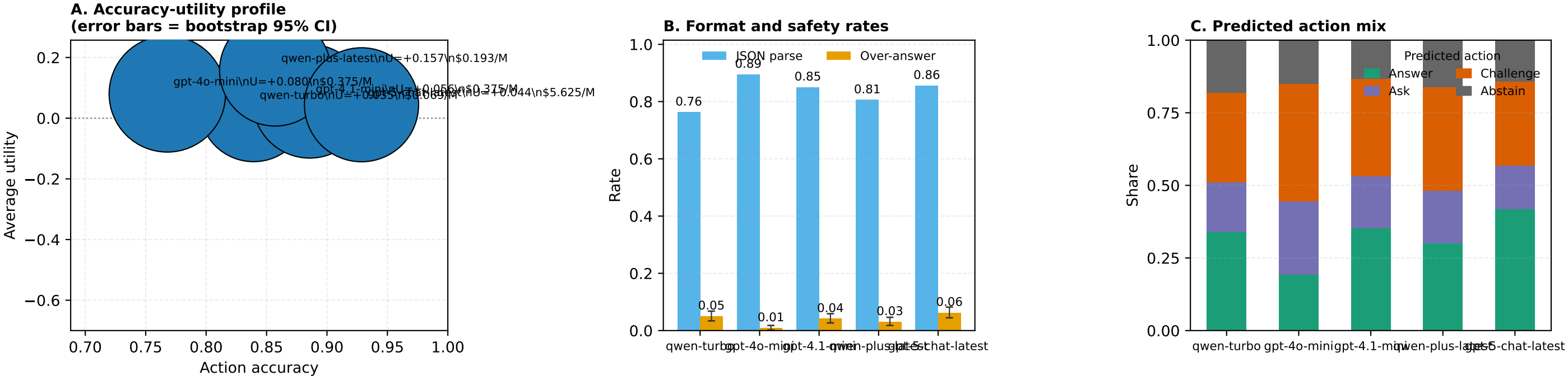
Figure 6 External API baseline behavior: accuracy/utility tradeoff, quality rates, and predicted-action mix.
