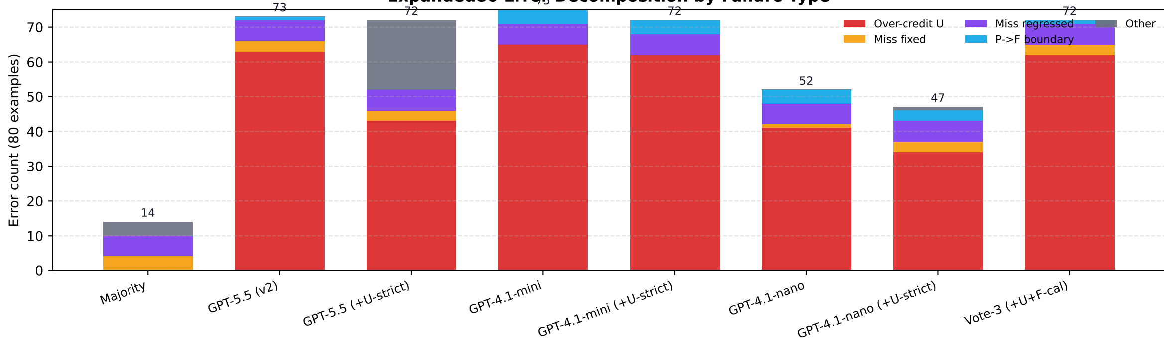
Expanded80 Error Decomposition by Failure Type
