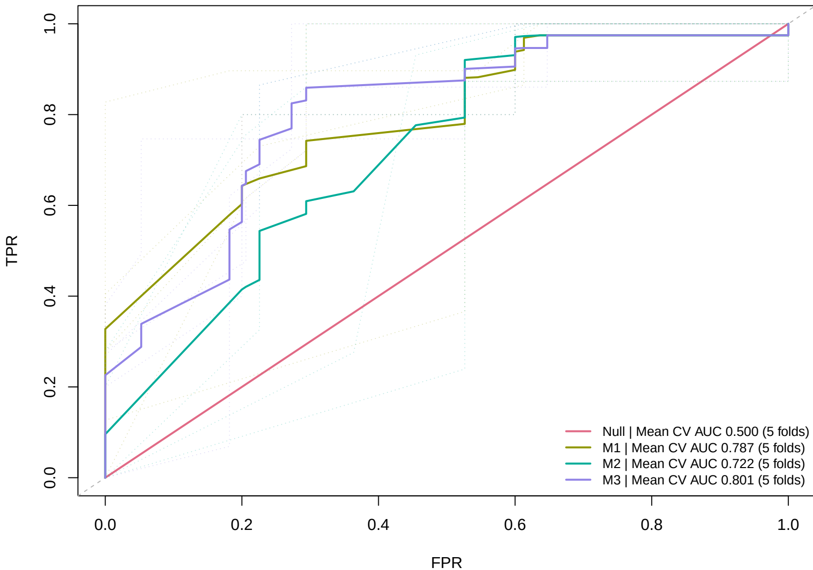
fivefold | species_equal | record_equal
