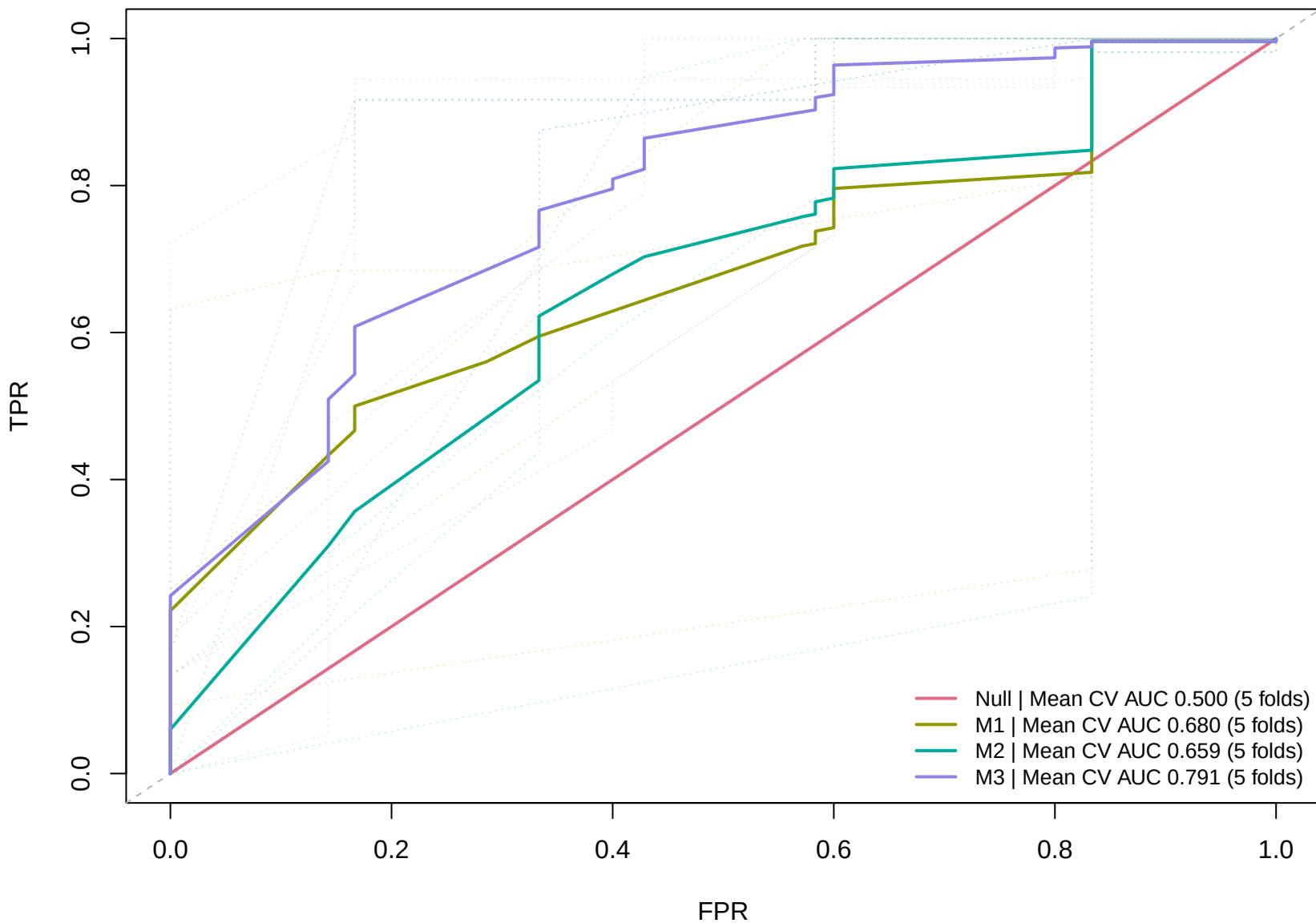
fivefold | record_equal | record_equal
