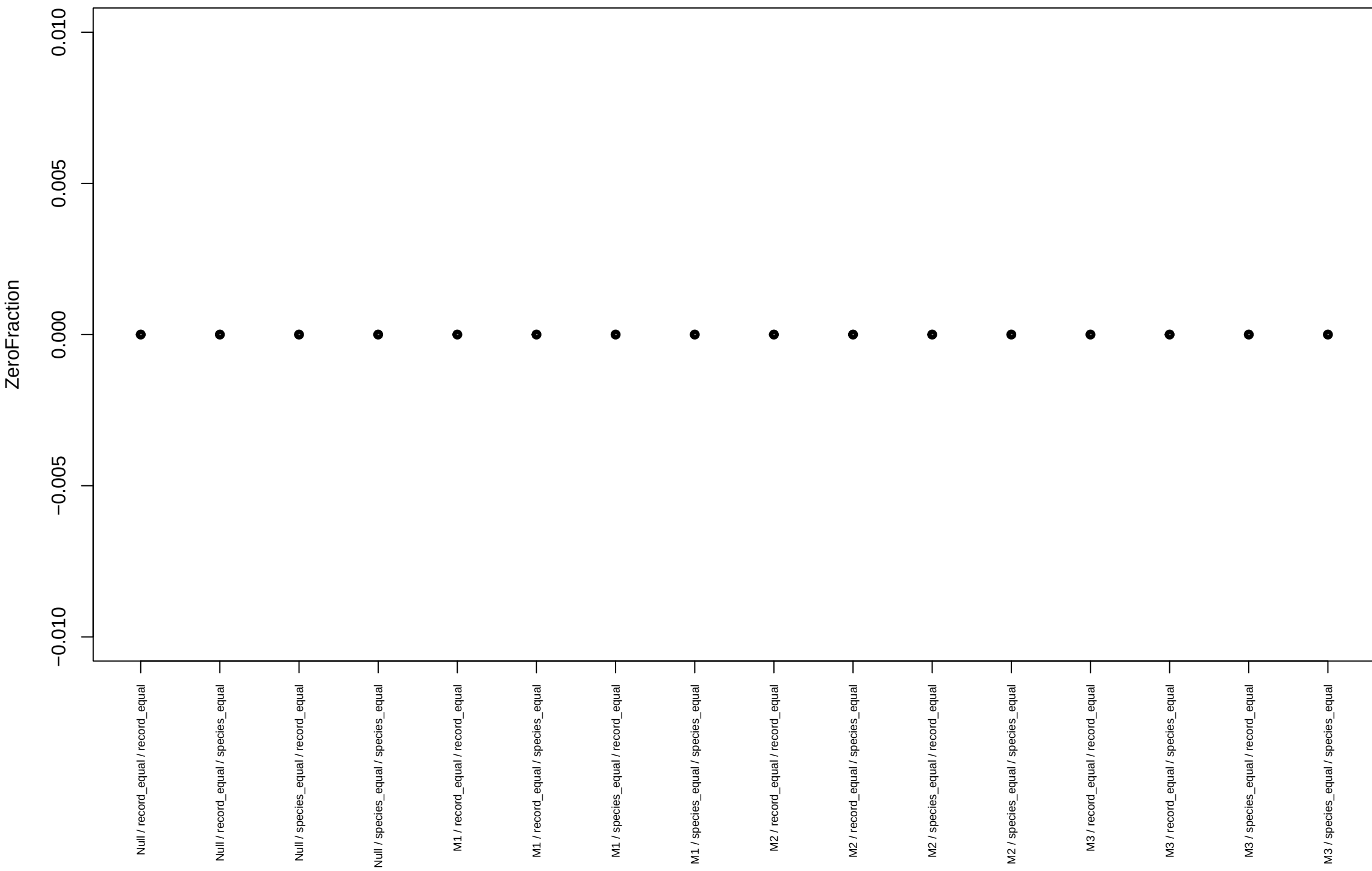
Training PPC exact ZeroFraction
