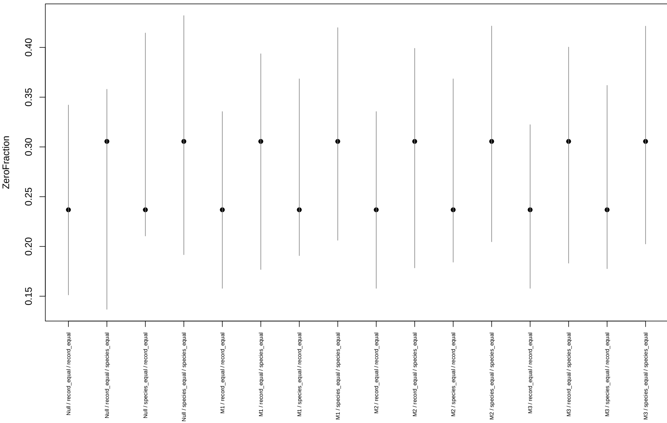
Training PPC classified ZeroFraction
