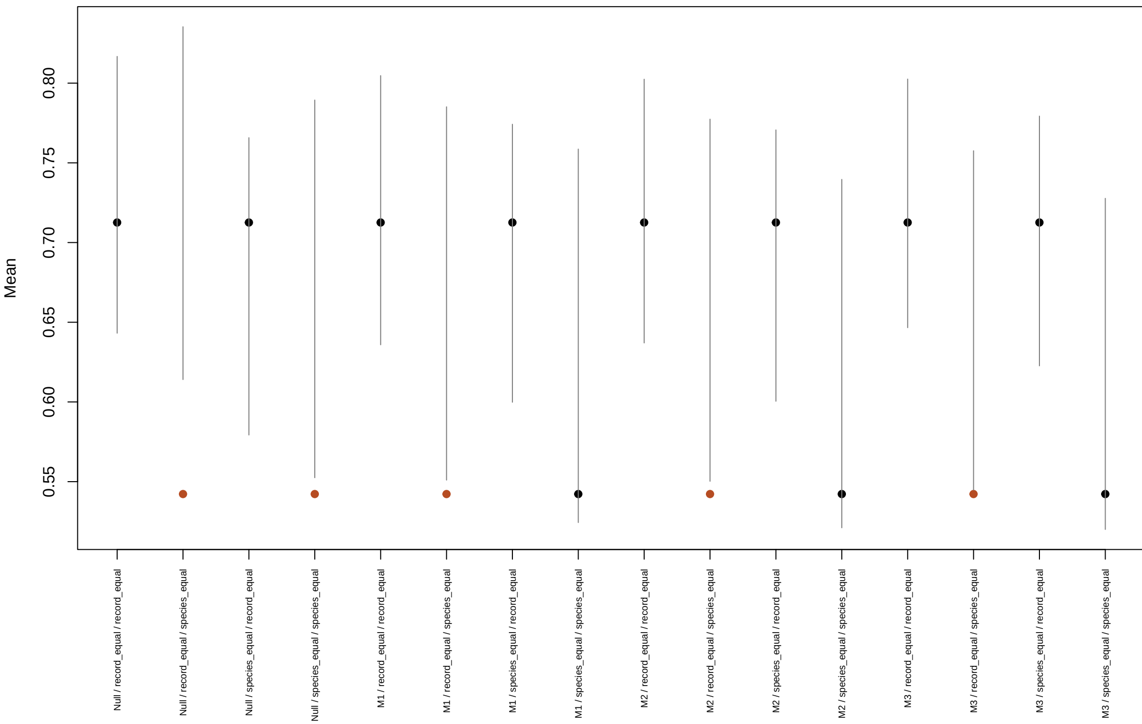
Training PPC count Mean
