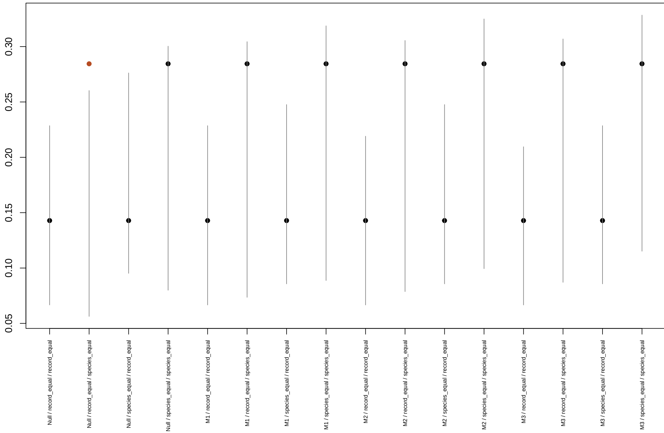
Training PPC count ZeroFraction
