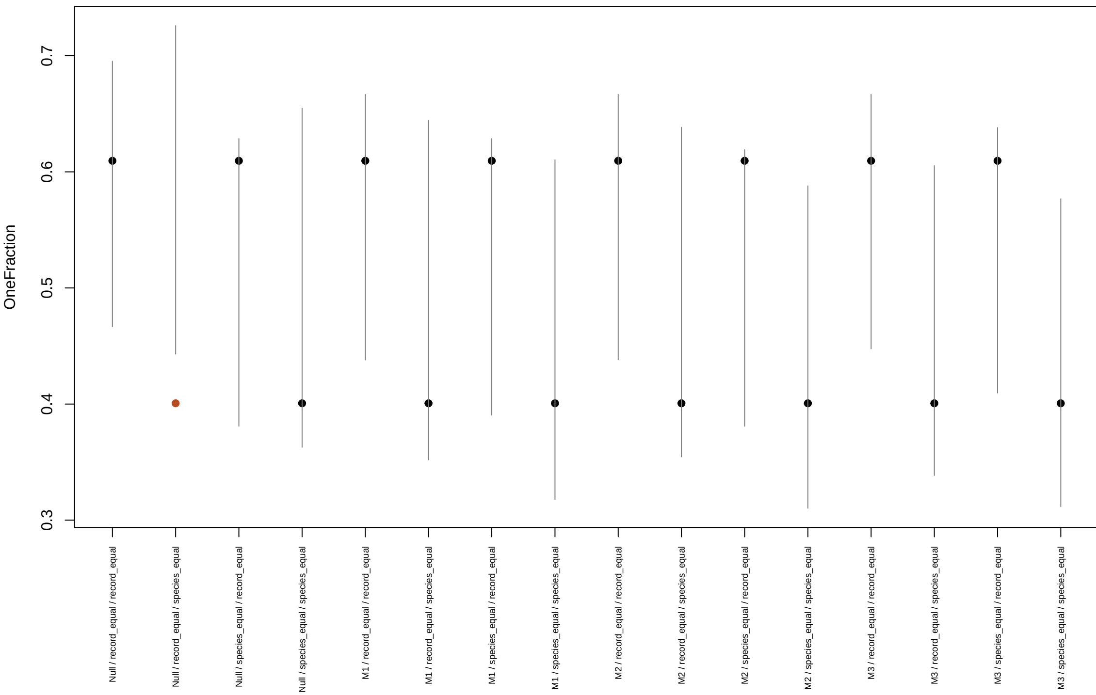
Training PPC count OneFraction
