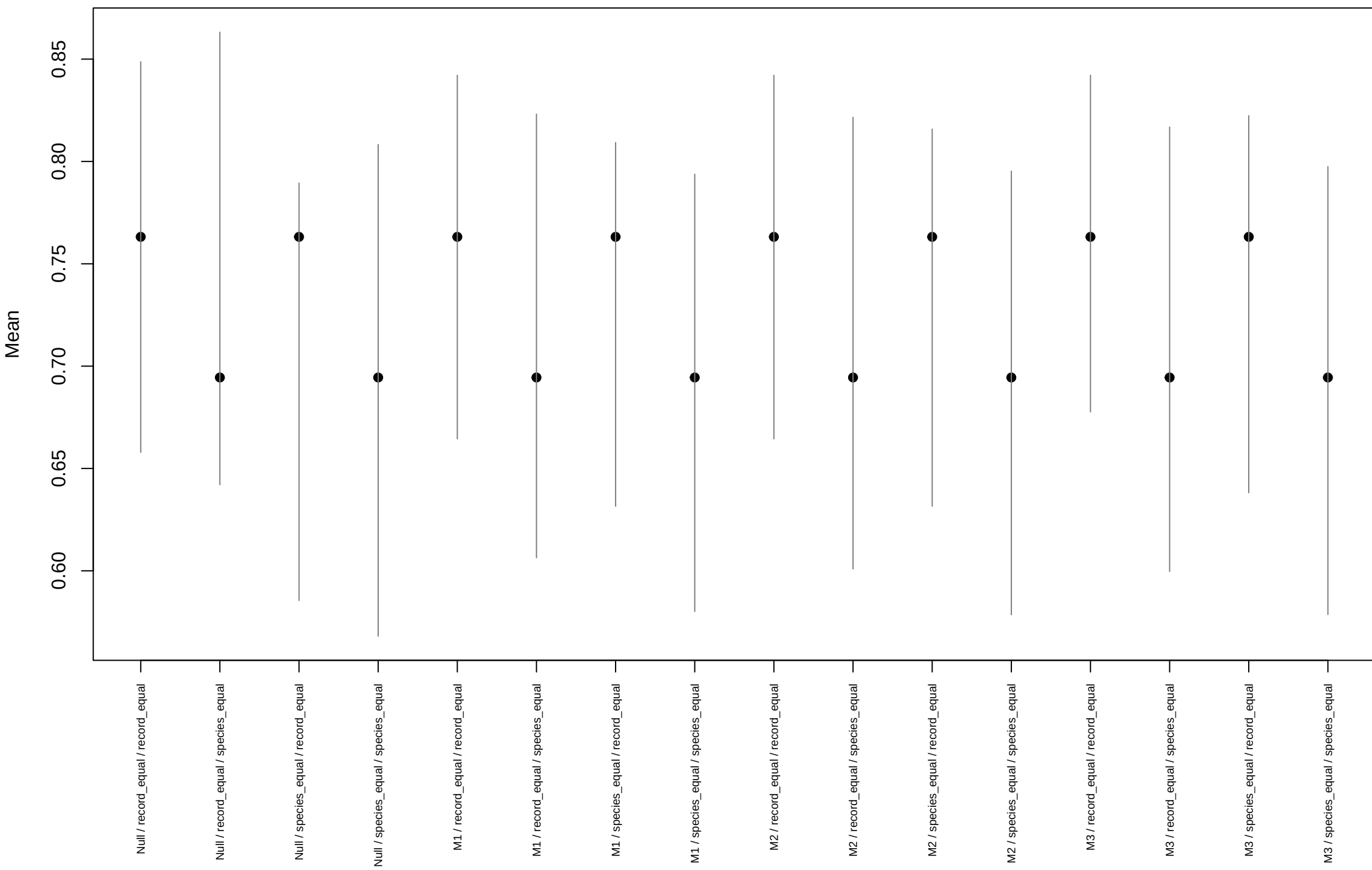
Training PPC classified Mean
