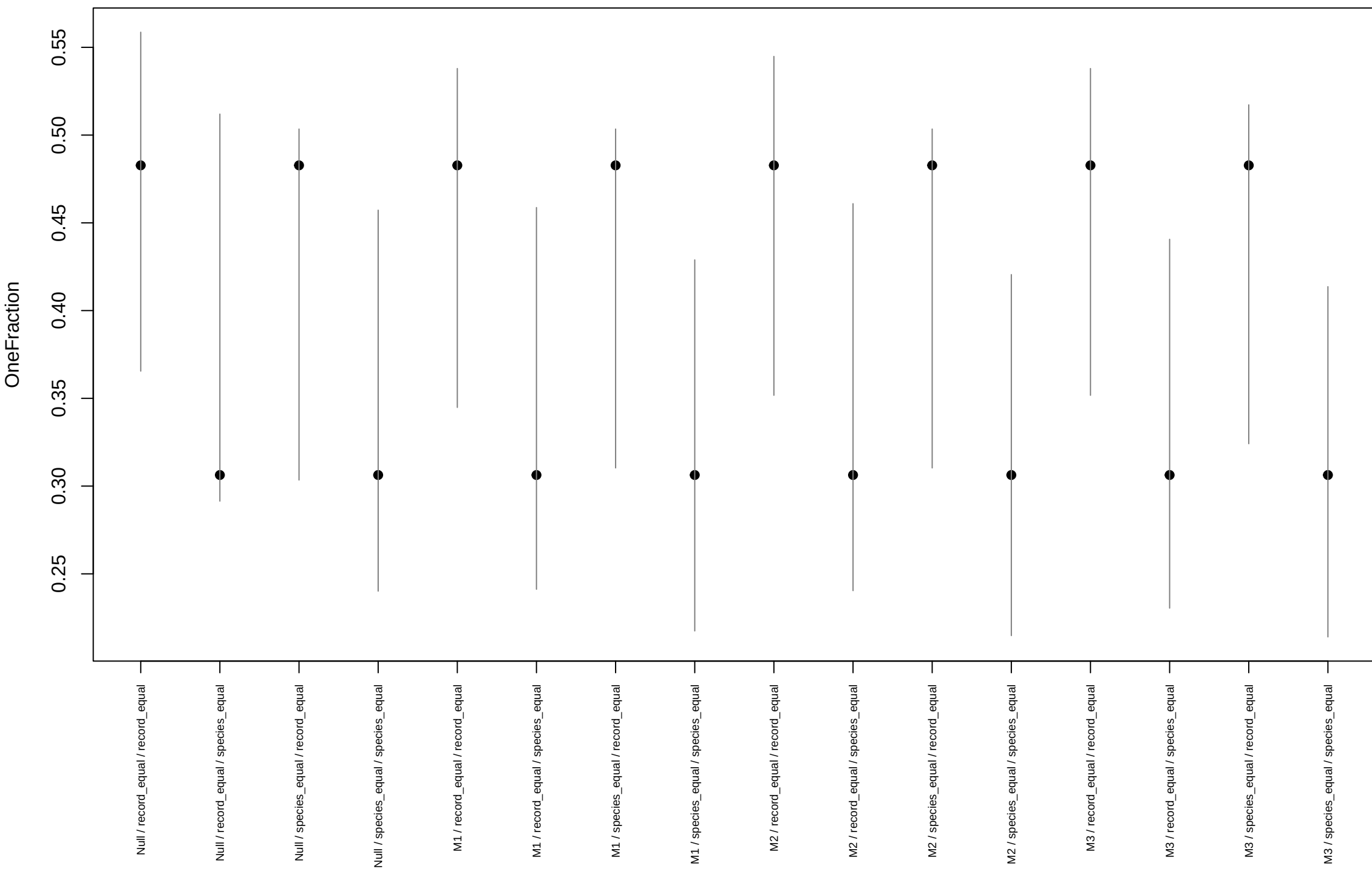
Training PPC all_point OneFraction
