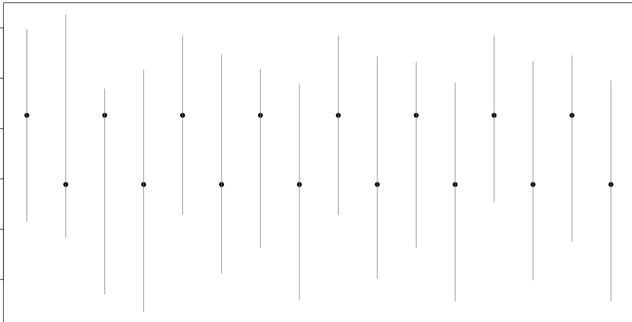
Training PPC classified OneFraction
