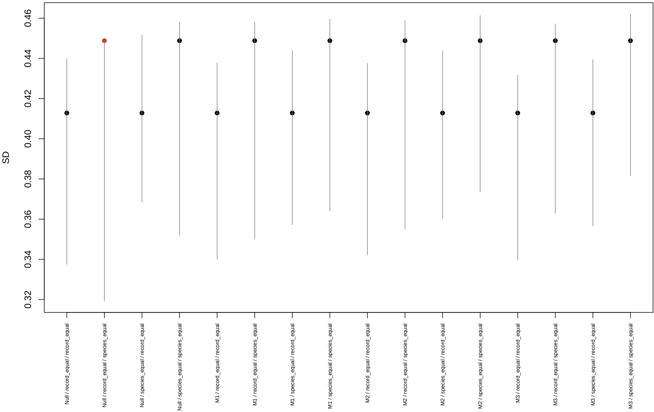
Training PPC count SD
