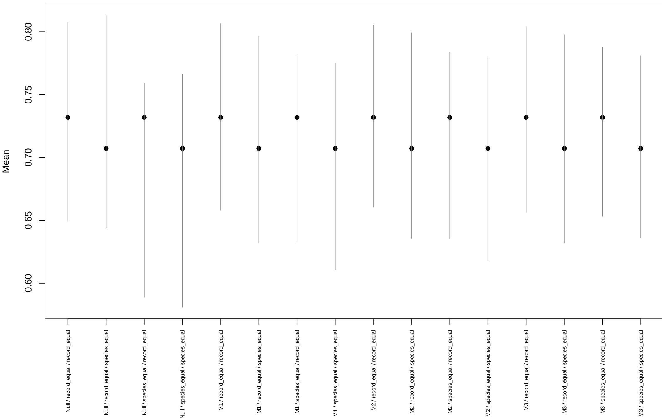
Training PPC exact Mean
