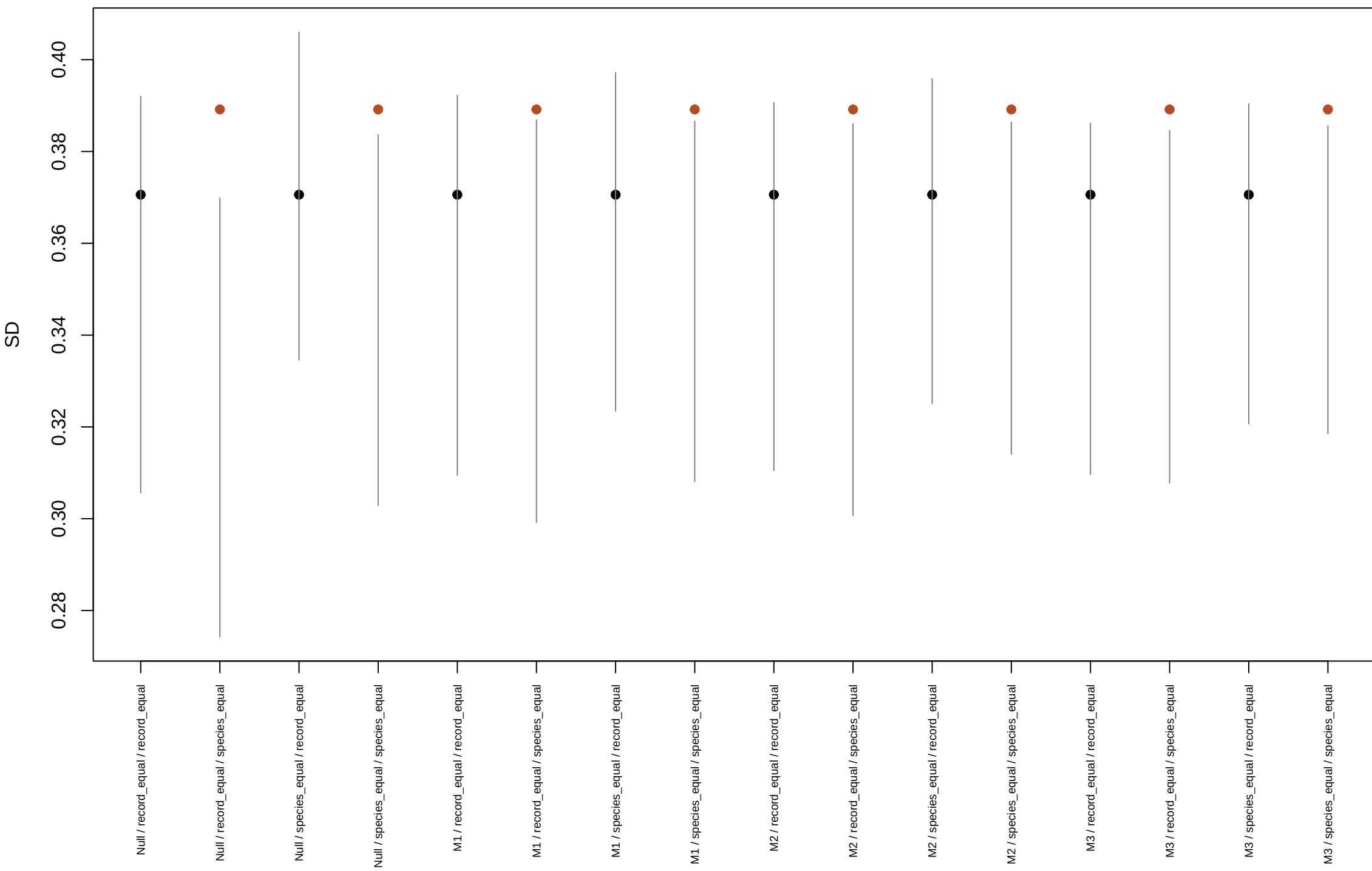
Training PPC all_point SD
