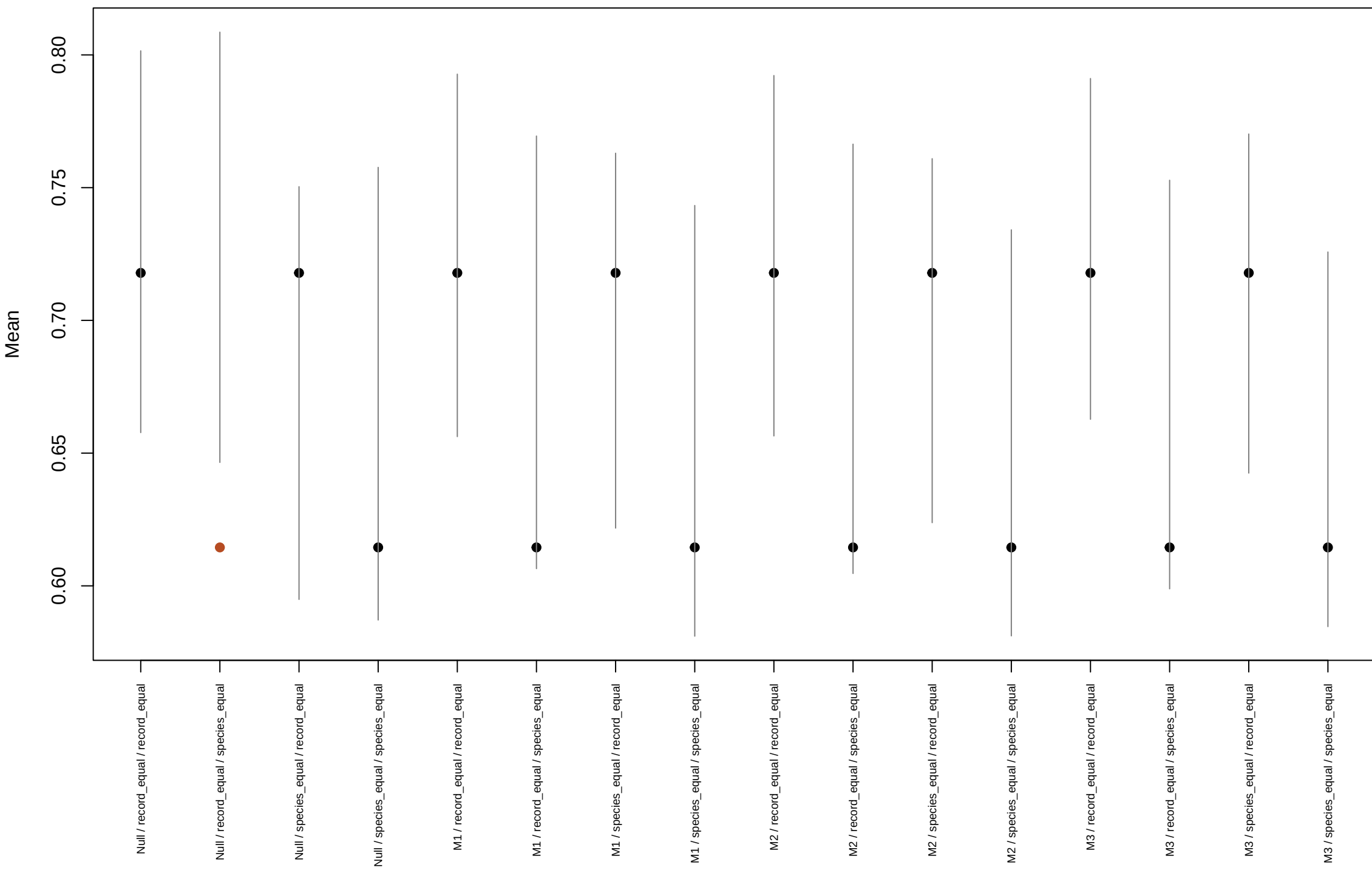
Training PPC all_point Mean
