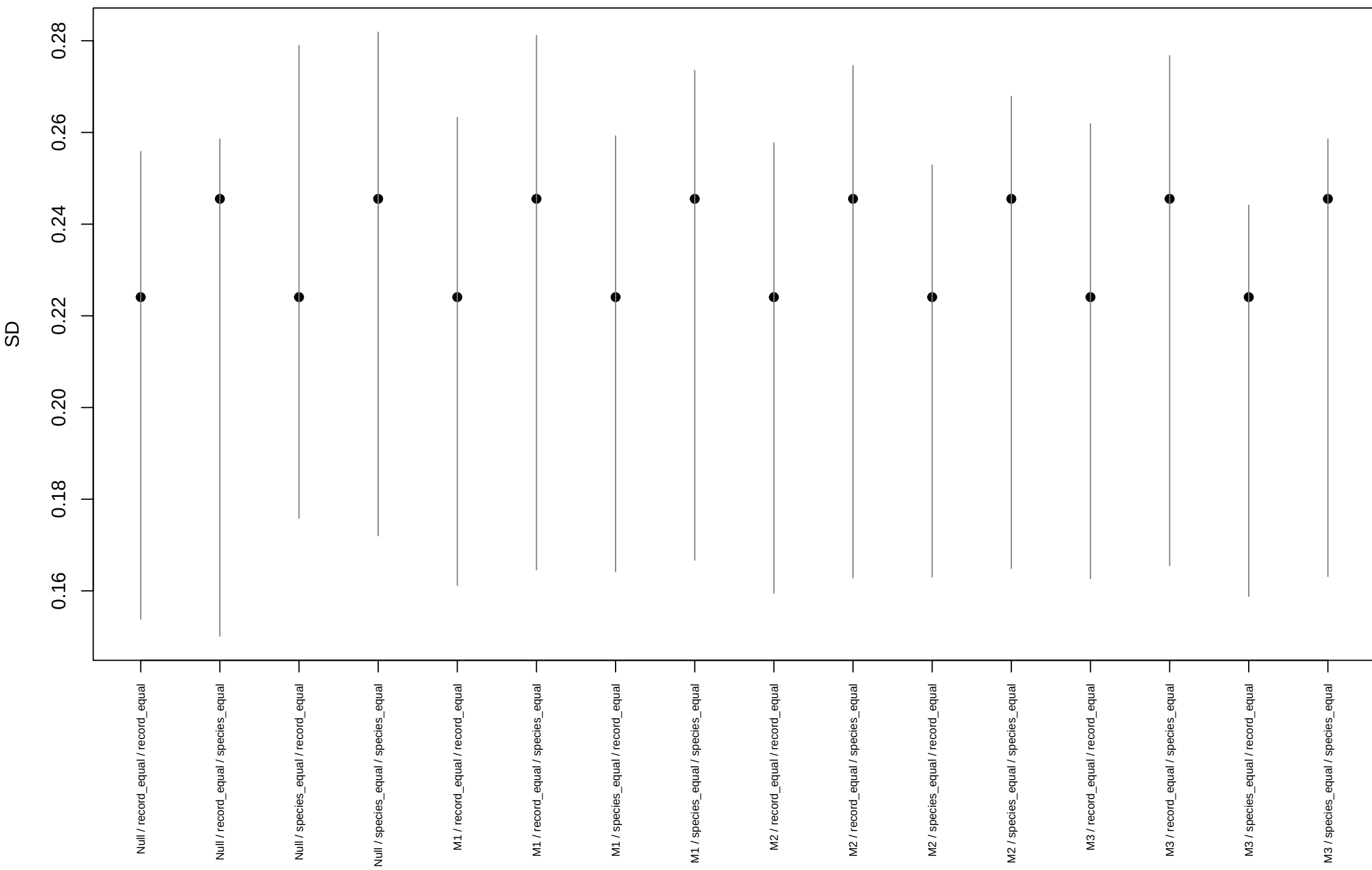
Training PPC exact SD
