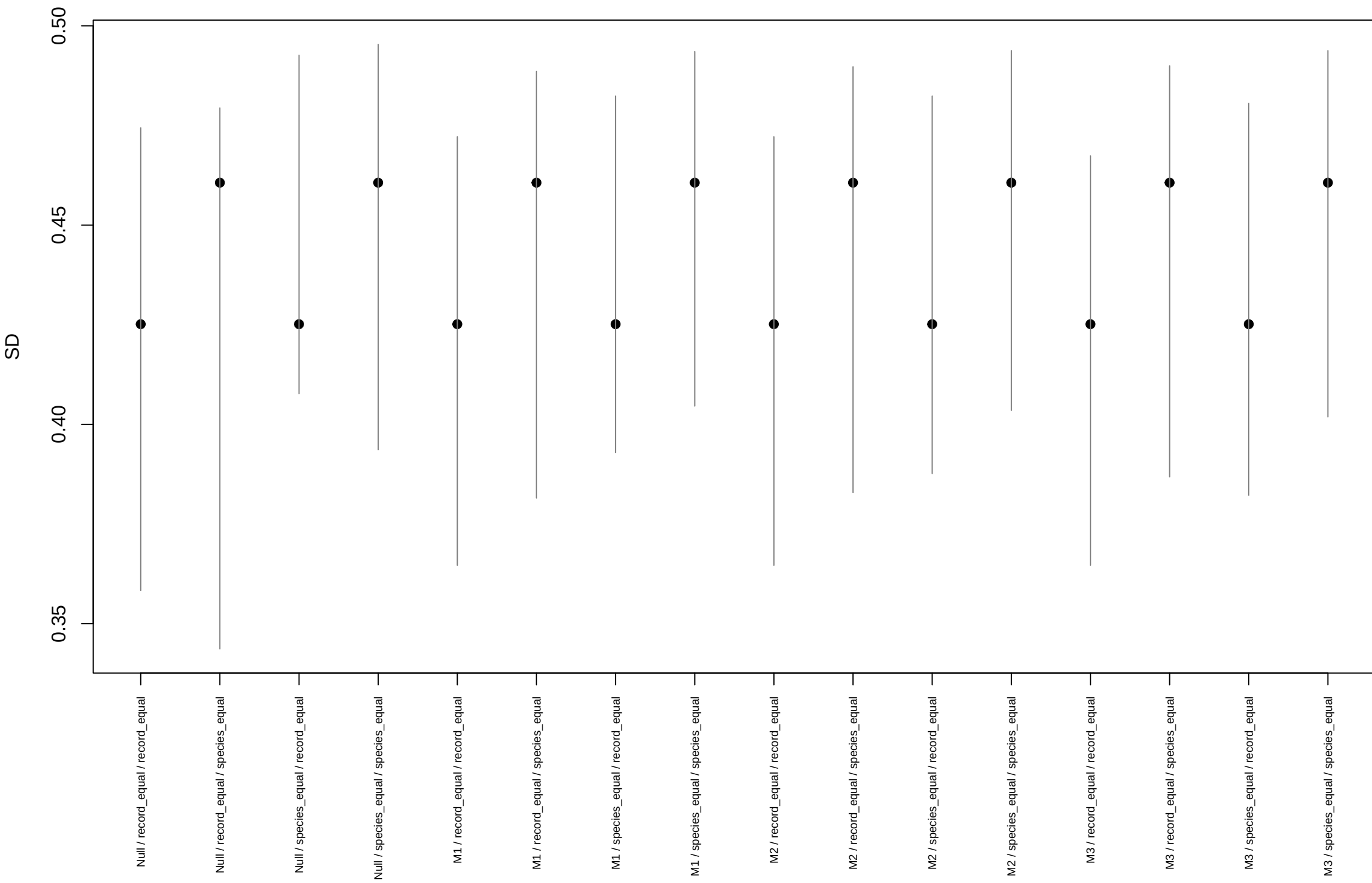
Training PPC classified SD
