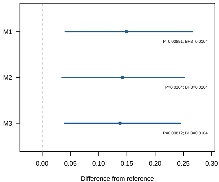
binary MeanLogScore
