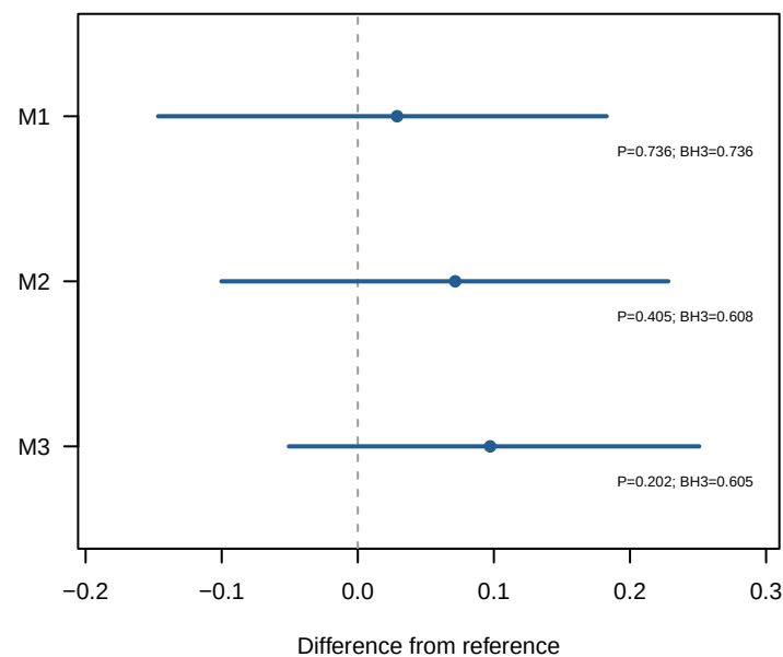
joint_bb MeanLogScore
