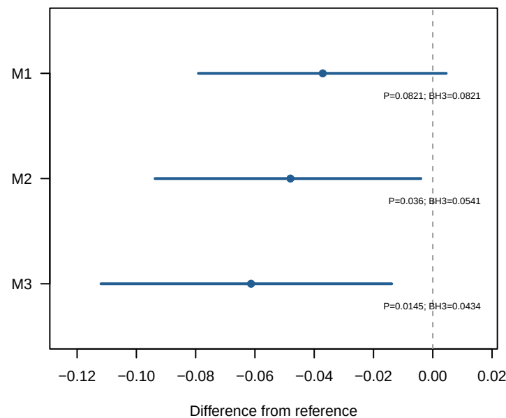
joint_bb RMSE
