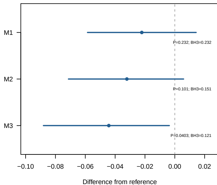
joint_bb MAE
