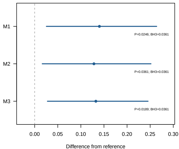
binary MeanLogScore
