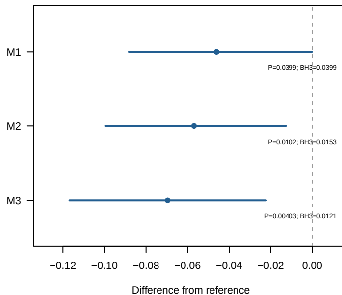
joint_bb RMSE
