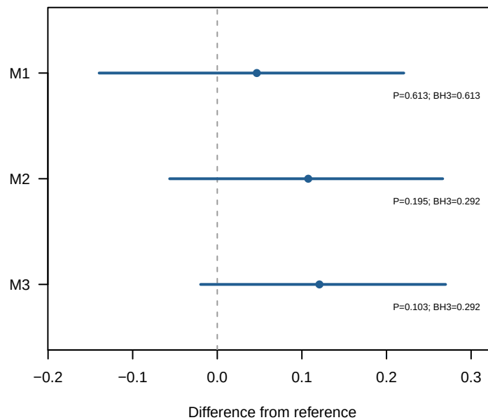
joint_bb MeanLogScore
