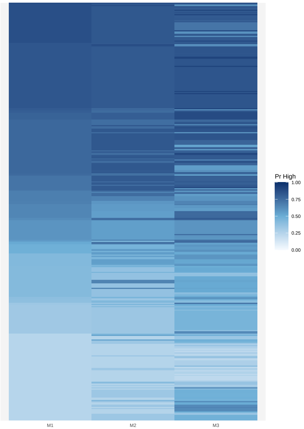
High-probability predictions across the 365-species panel Species ordered by M1 posterior High probability; Site151 is excluded from all model predictors
