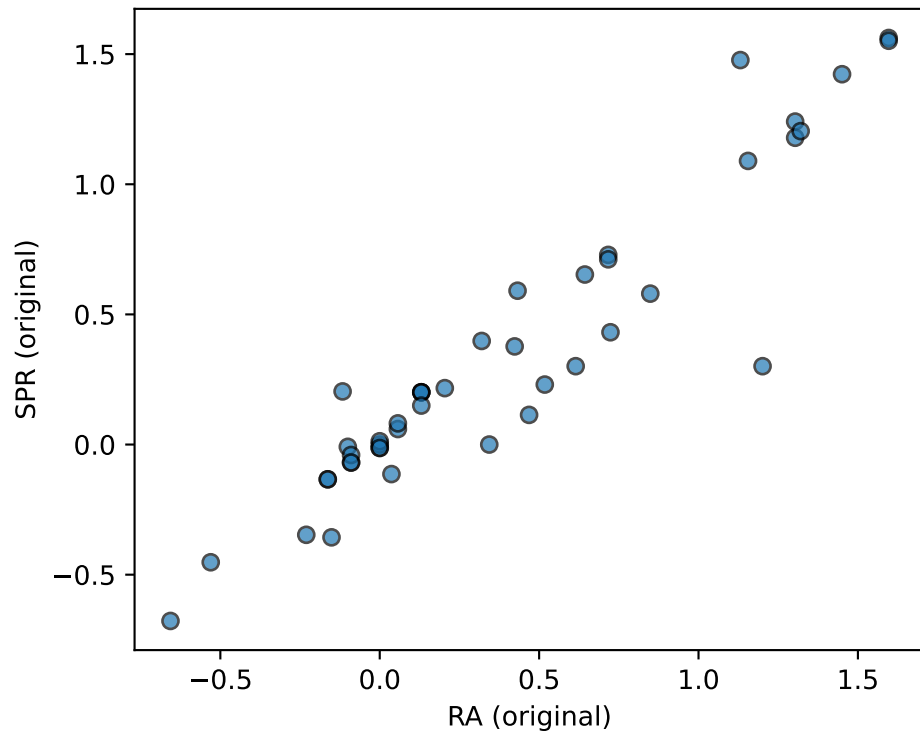
Before Calibration Pearson r=0.94
