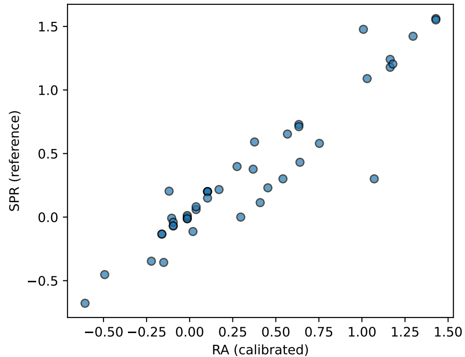
After Calibration Pearson r=0.94
