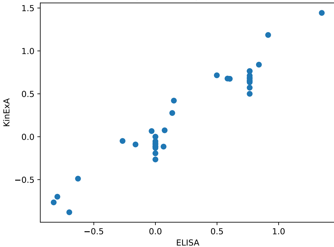
ELISA vs KinExA r=0.97 , p=0.0001 , q=0.00018 , n=37
