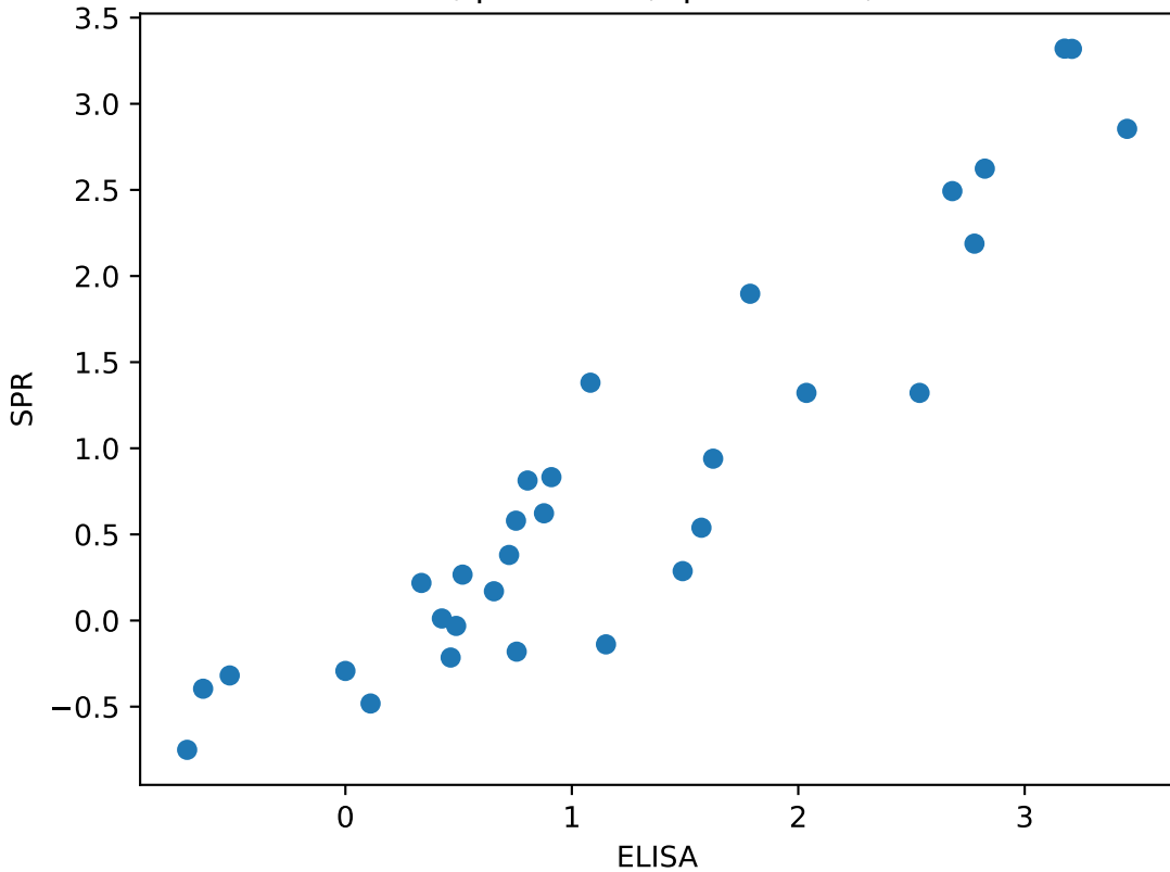
ELISA vs SPR r=0.93 , p=0.0001 , q=0.00018 , n=31
