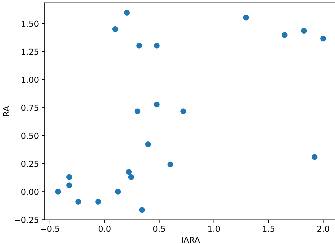
IARA vs RA r=0.54 , p=0.0054 , q=0.0085 , n=23
