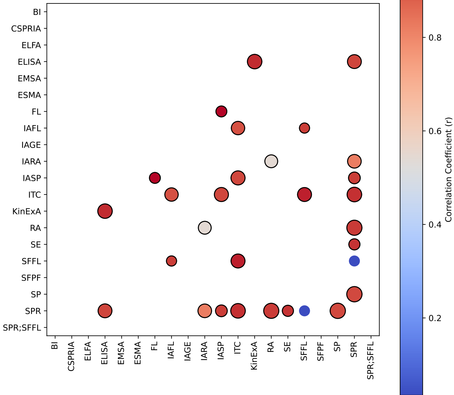
Correlation Bubble Plot (Size = sample size, Color = correlation, Black edge = p < 0.05 )
