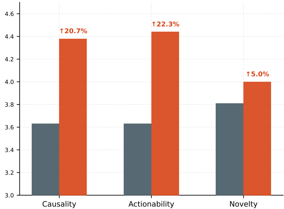
Exploratory Tasks (High Diff)
