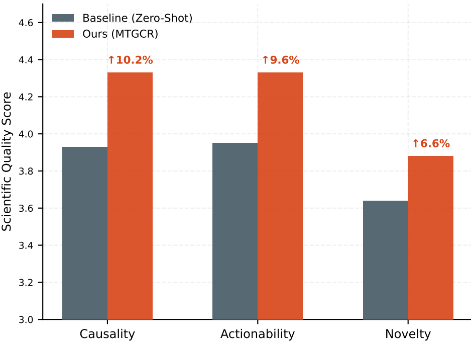
Overall Performance (N=42)
