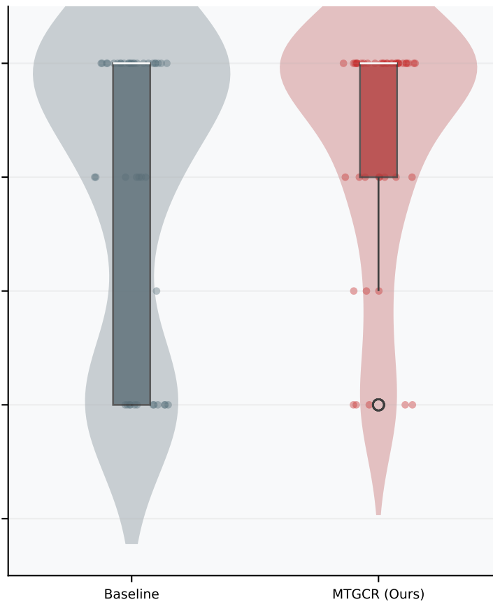
Engineering Actionability
