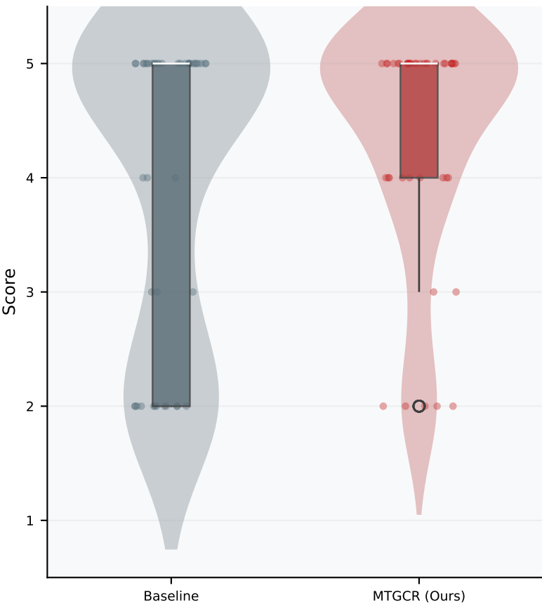
Causal Rigor
