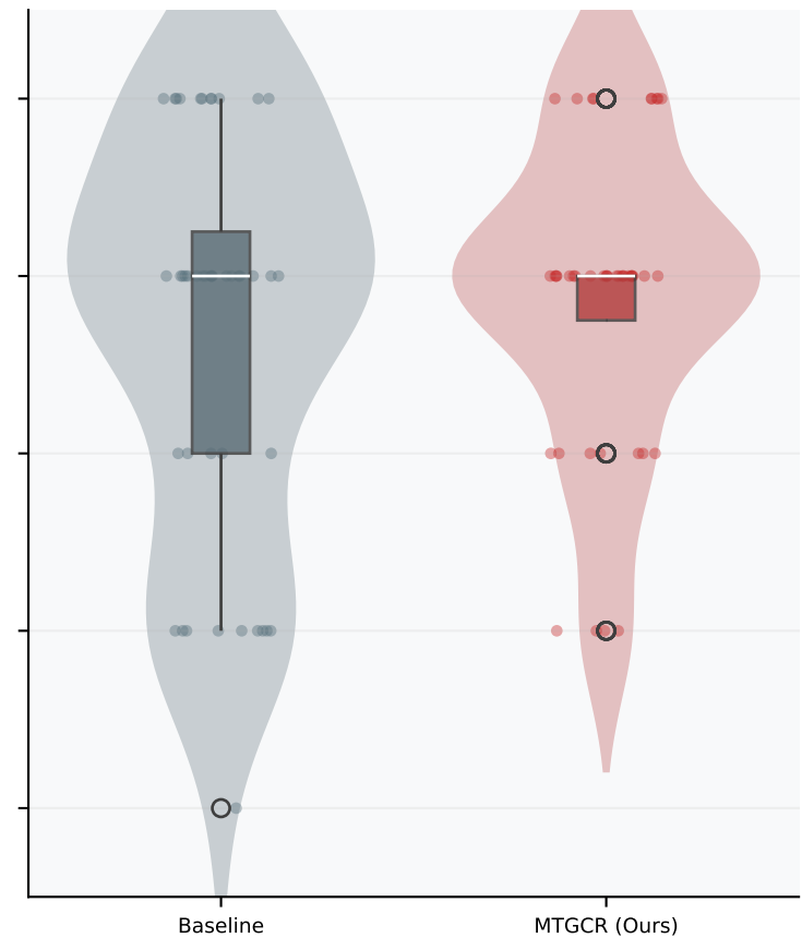
Scientific Novelty
