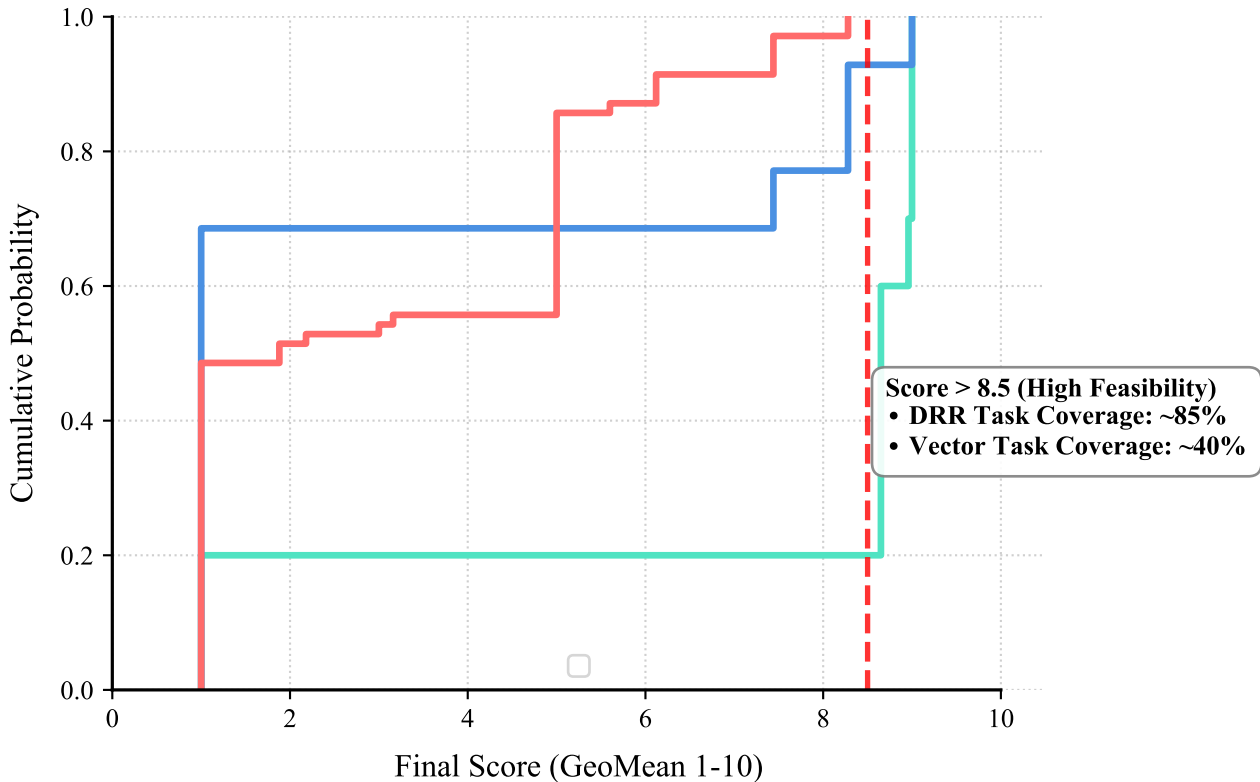
Empirical CDF of Final Scores (Strict Dominance)
