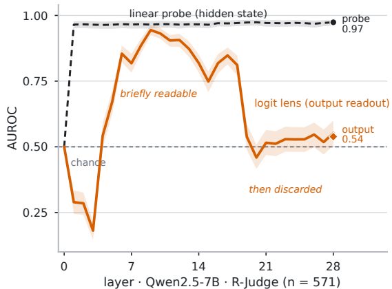
(a) “attack?” decodability across layers
