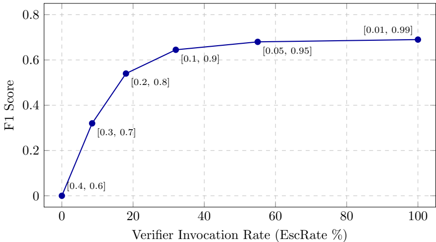
Accuracy-Cost Trade-off (Gating Sweep)
