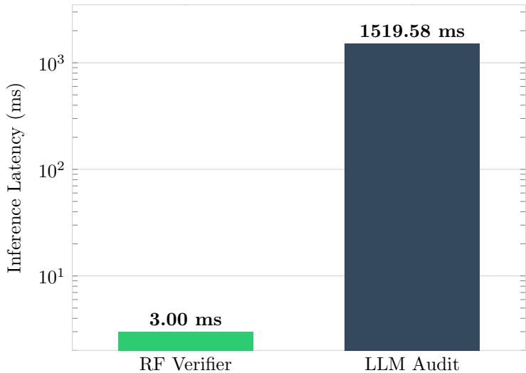
Latency Comparison (Log Scale)
