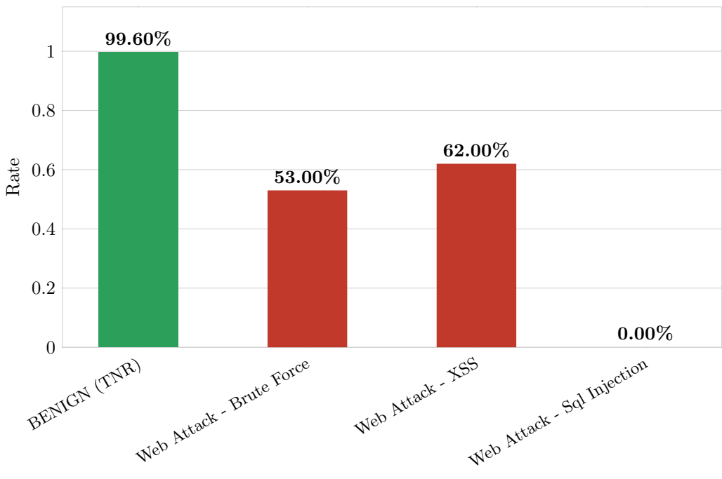
Detection Coverage by Class (Gated Pipeline)
