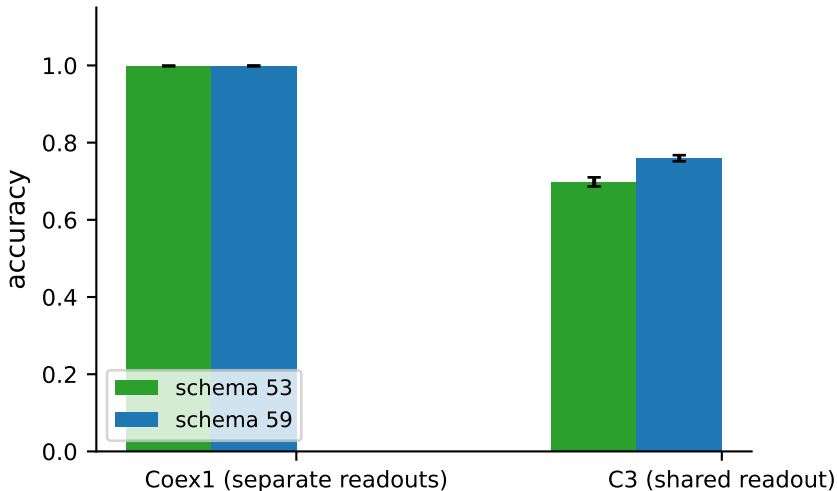
Co-grokking (final accuracy): 10/10 vs 0/10 (10 seeds)
