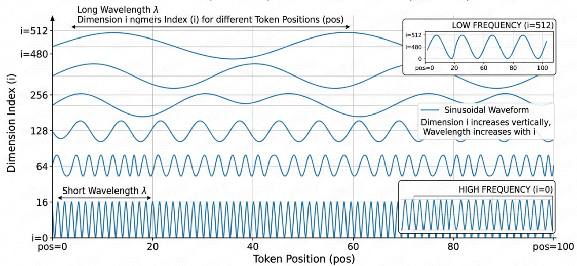
Figure 1.2: Frequency Spectrum of Sinusoidal Positional Encoding
