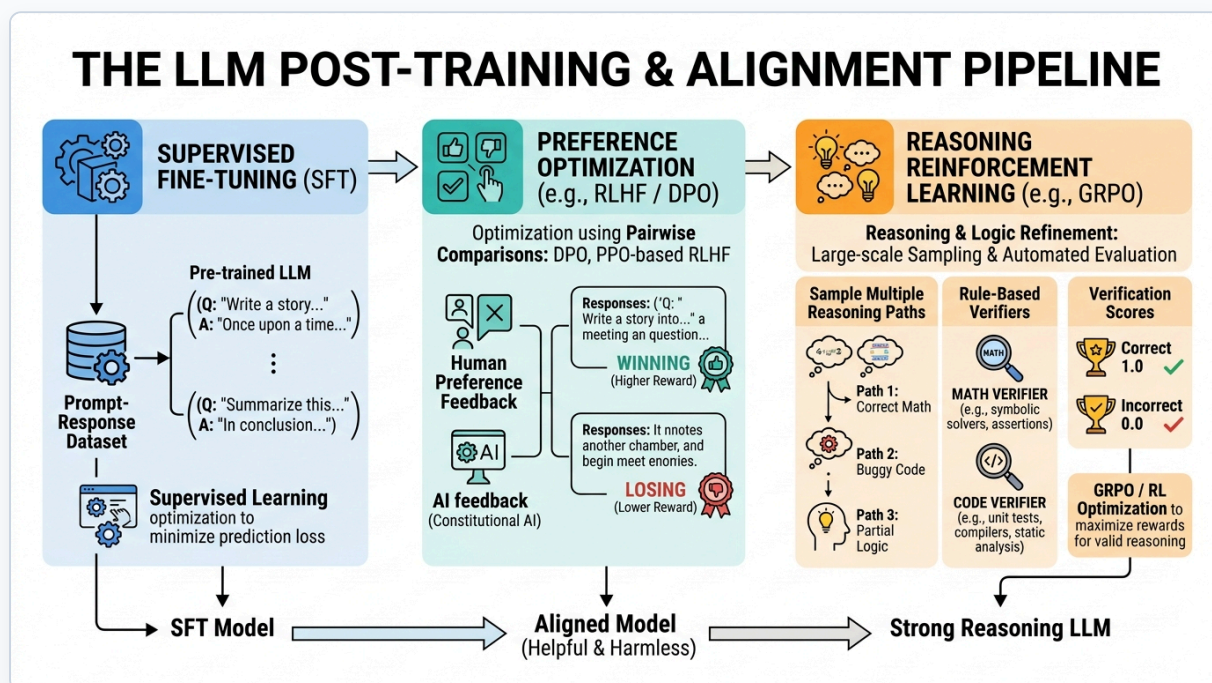
Figure 7.1: The Post-Training Alignment Hierarchy: SFT, RLHF, and GRPO
