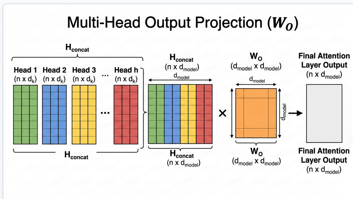
Figure 3.2: Multi-Head Concatenation and Output Projection W_O
