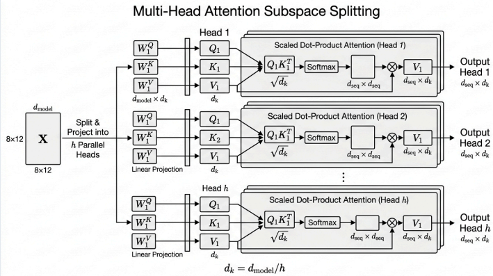
Figure 3.1: Multi-Head Attention Subspace Splitting
