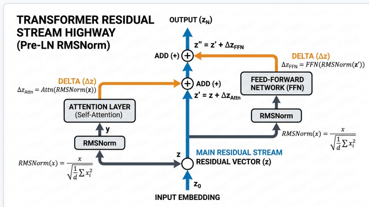
Figure 4.1: Residual Stream Highway Architecture
