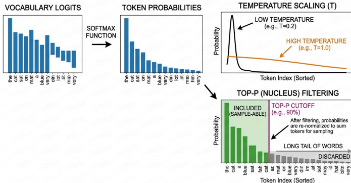
Figure 6.3: Nucleus Top-p Probability Mass Cutoff
