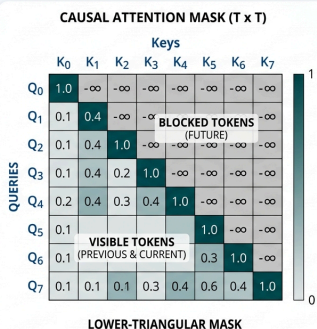
Figure 3.3: Causal Attention Masking Matrix Arithmetic
