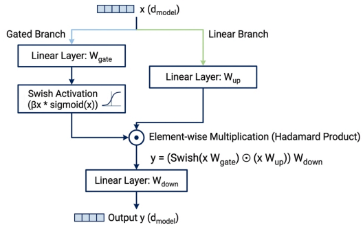
Figure 5.2: SwiGLU Multiplicative Gating Mechanism
