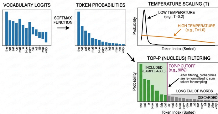
Figure 6.2: Temperature Entropy Calibration
