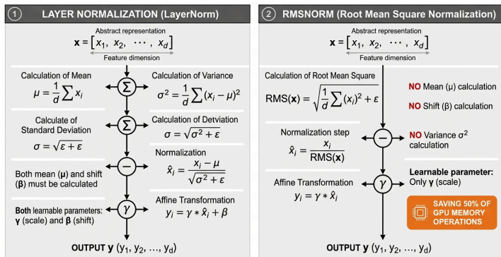
Figure 4.2: Layer Normalization vs RMSNorm Architecture
