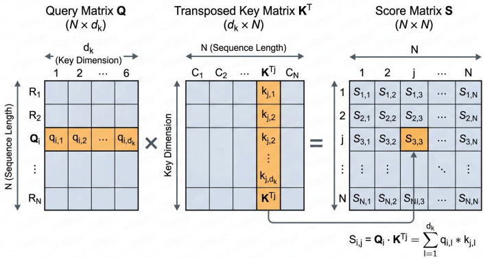
Figure 2.2: Raw Compatibility Scoring Matrix Multiplication
