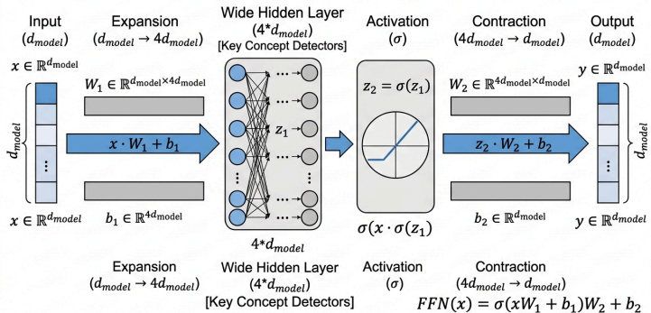
Figure 5.1: Two-Layer Feed-Forward Network (FFN) Expansion
