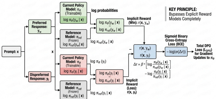
Figure 7.3: Direct Preference Optimization (DPO) Loss Architecture
