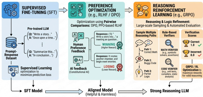
Figure 7.1: The Post-Training Alignment Hierarchy: SFT, RLHF, and GRPO
