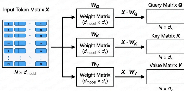
Figure 2.1: Query, Key, and Value Linear Projections
