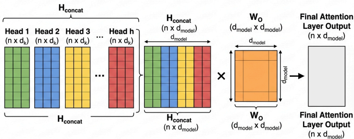
Figure 3.2: Multi-Head Concatenation and Output Projection W_O
