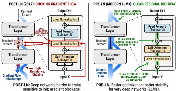
Figure 4.3: Post-LN vs Pre-LN Architectural Flow
