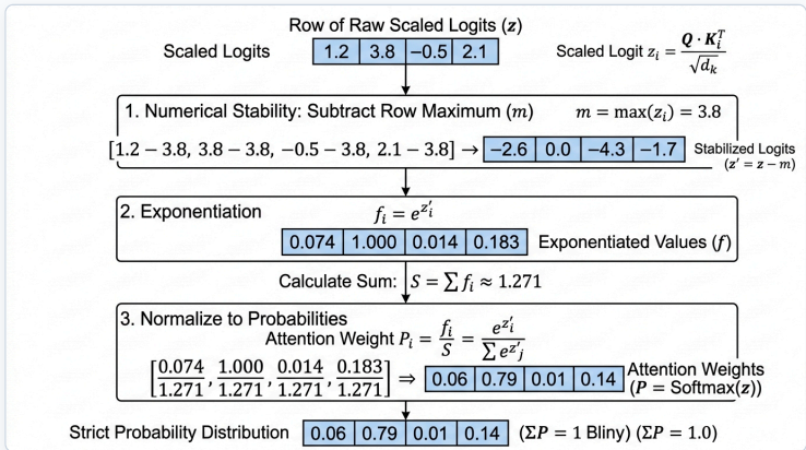
Figure 2.4: Softmax Row-wise Probability Normalization
