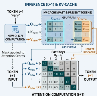
Figure 3.3: Causal Attention Masking Matrix Arithmetic
