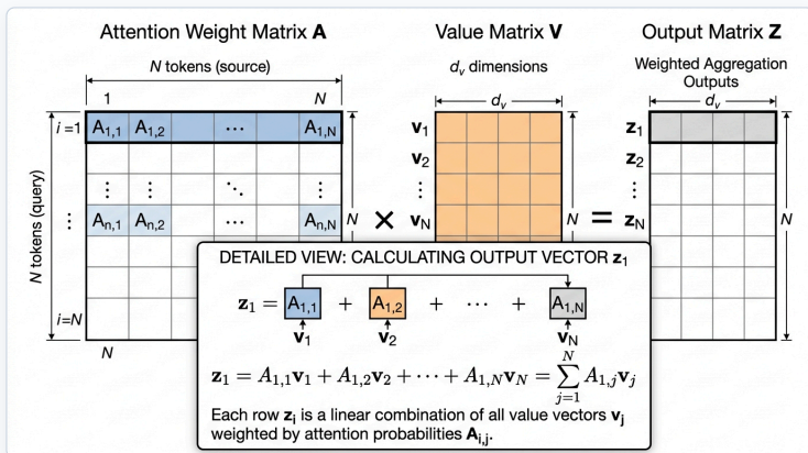
Figure 2.5: Weighted Value Aggregation and Output Representation
