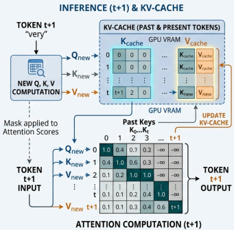
Figure 3.4: Autoregressive KV-Cache VRAM Dynamic Memory
