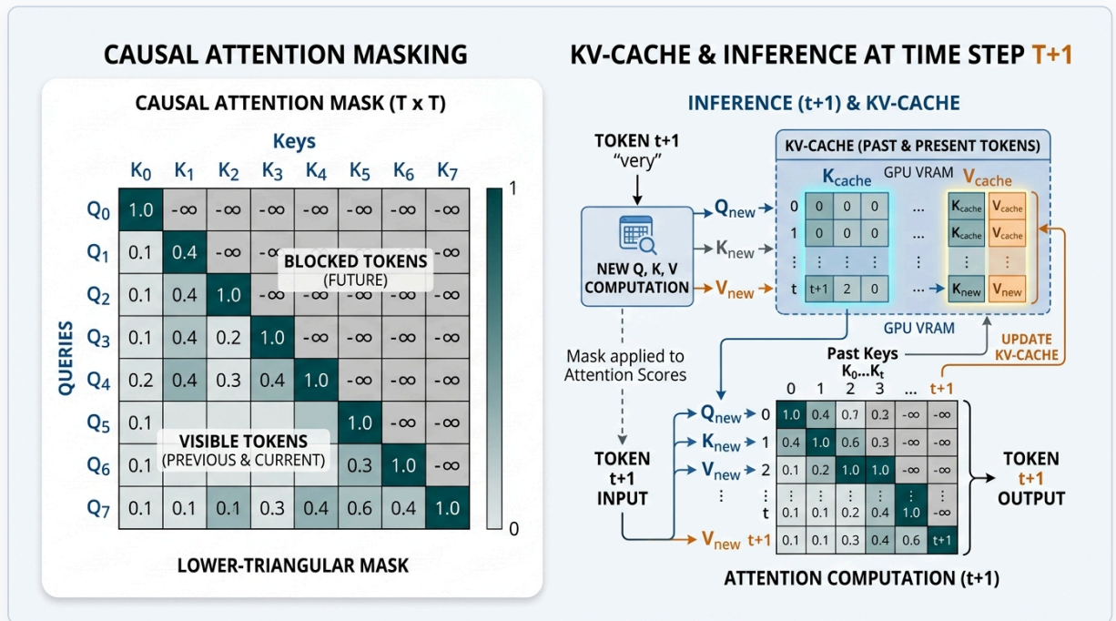
Figure 3.3: Causal Attention Masking Matrix Arithmetic
