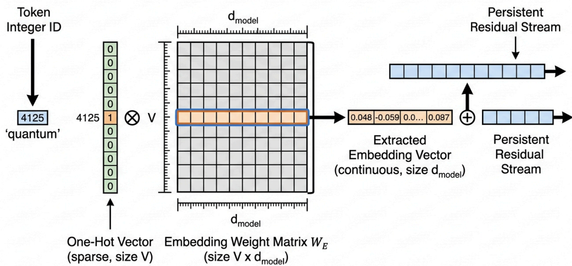
Figure 0.2: Token Embedding Matrix Lookup and Residual Stream Projection
