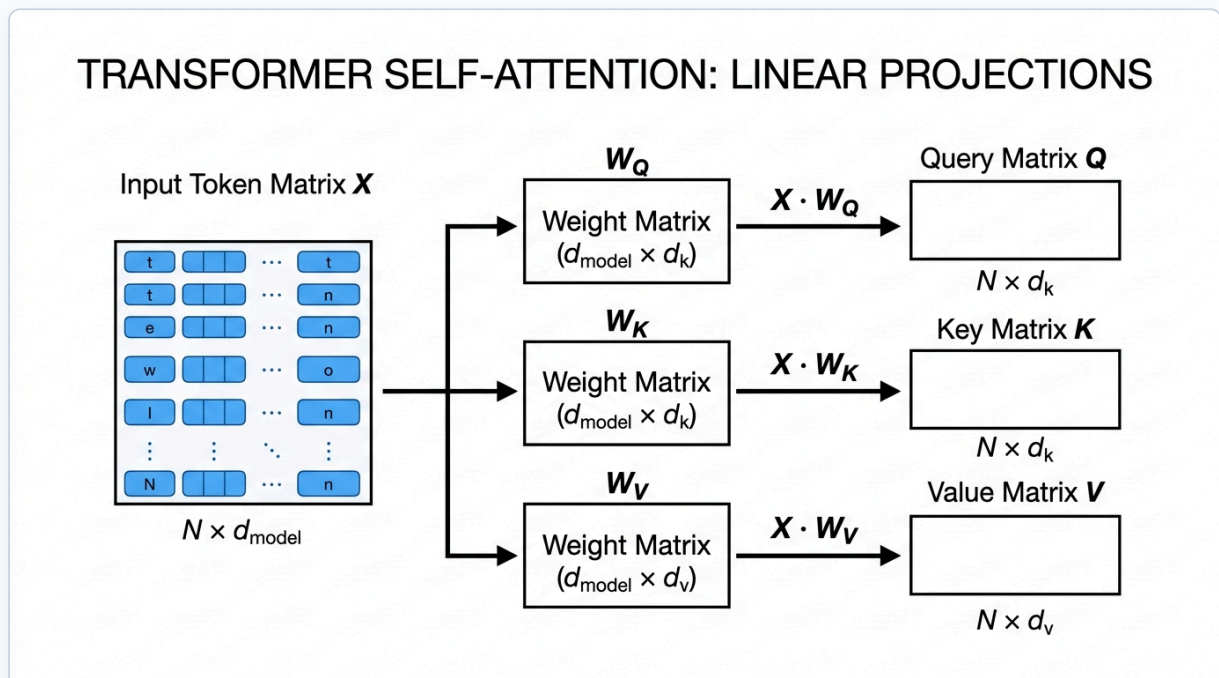
Figure 2.1: Query, Key, and Value Linear Projections
