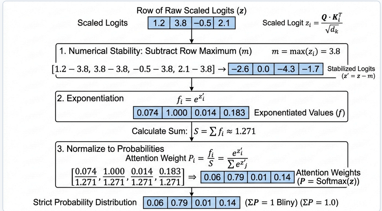
Figure 2.4: Softmax Row-wise Probability Normalization
