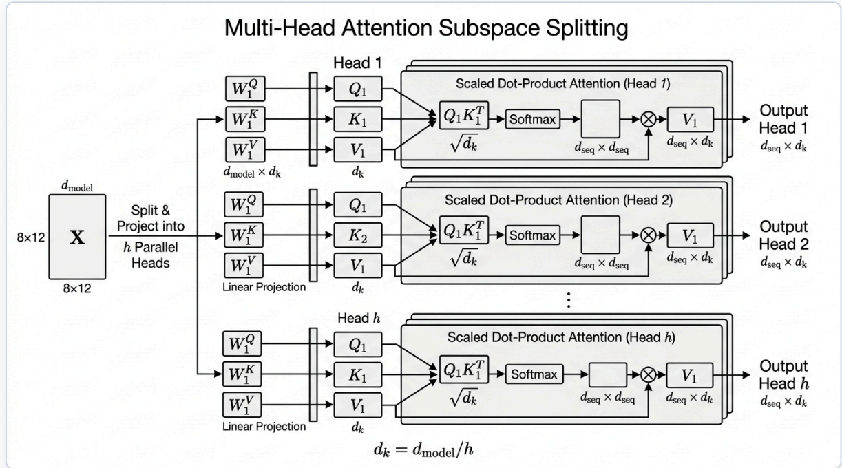
Figure 3.1: Multi-Head Attention Subspace Splitting
