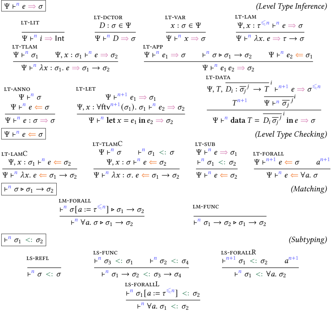
Fig. 3. Level-based declarative type system
