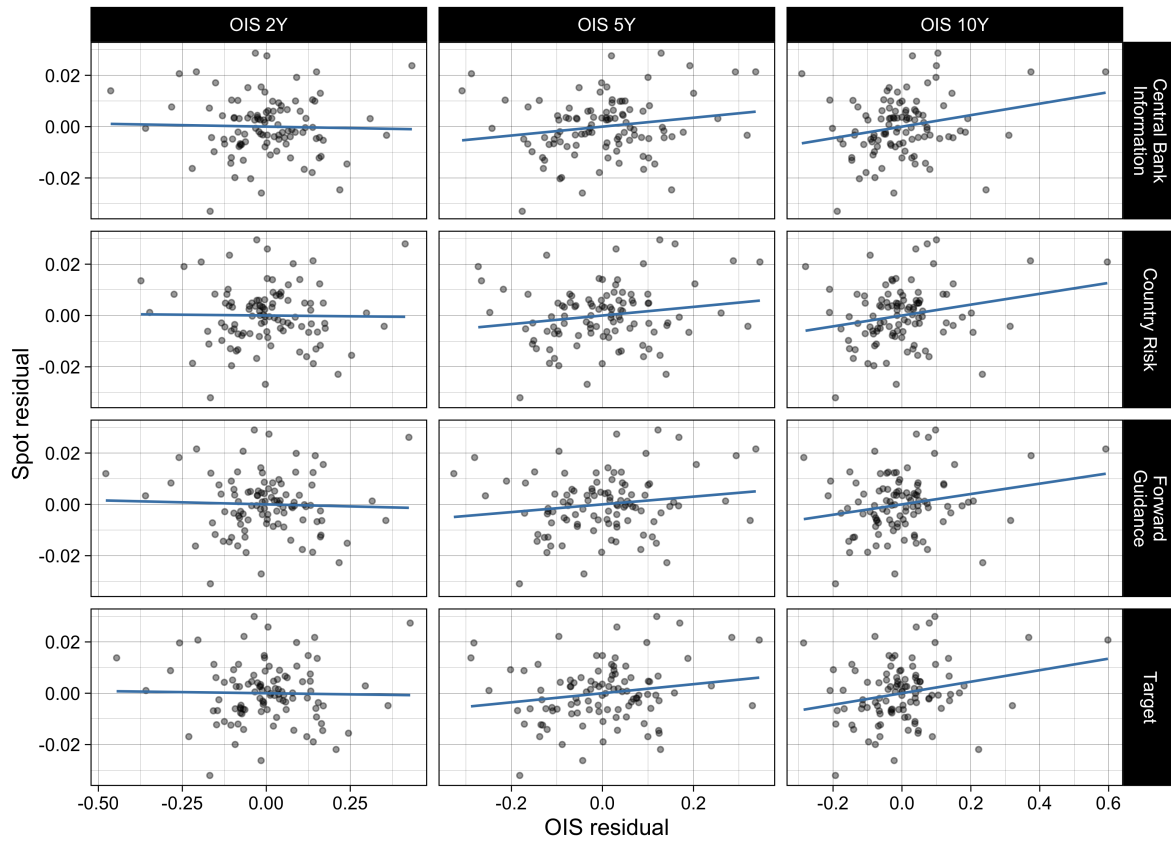
Residual-on-residual: spot vs OIS
