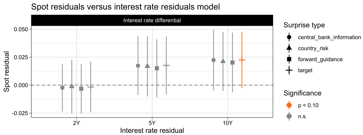
Figure 4: Spot residuals versus interest rate residuals model
