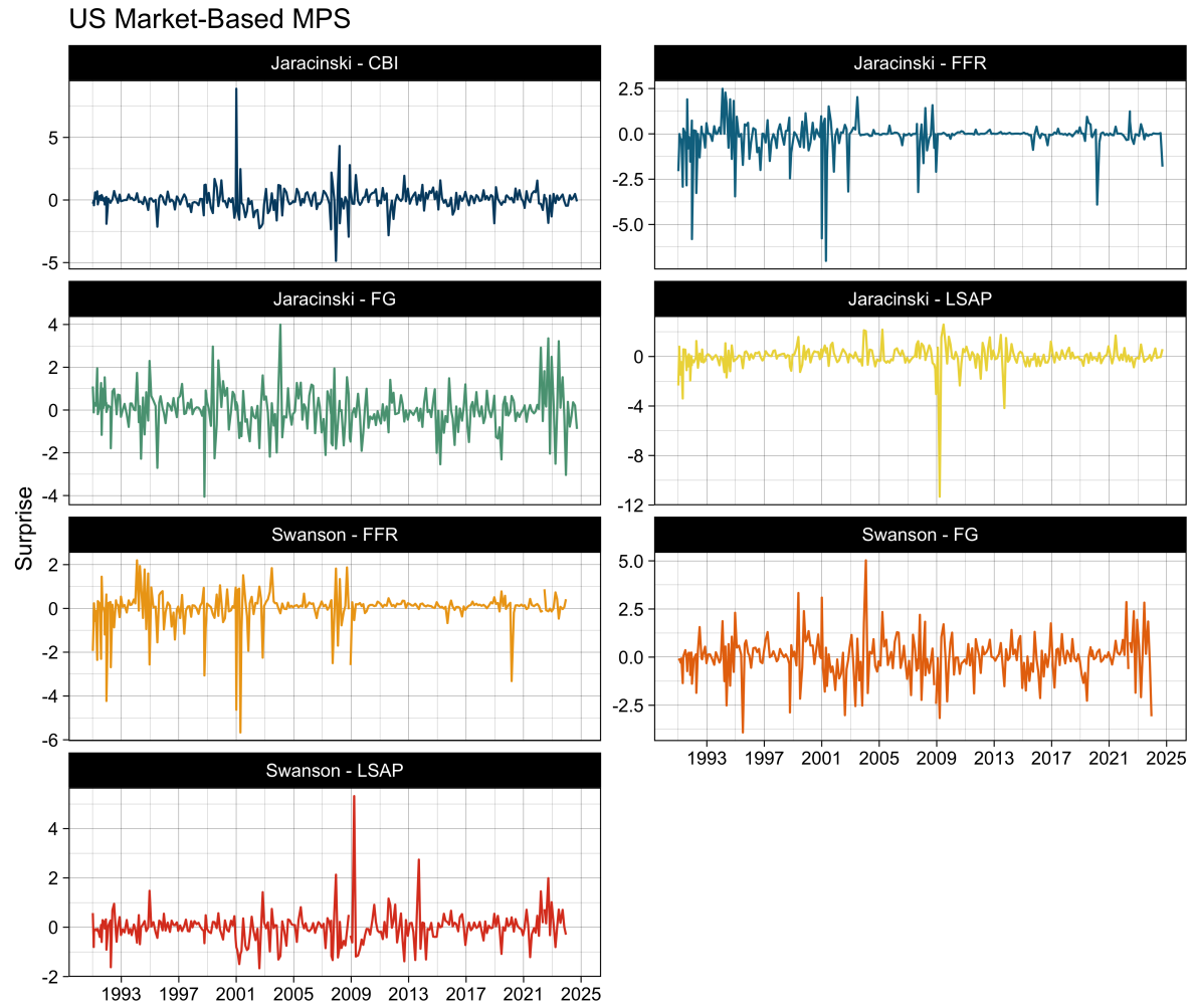
Figure A2: US monetary policy surprises
