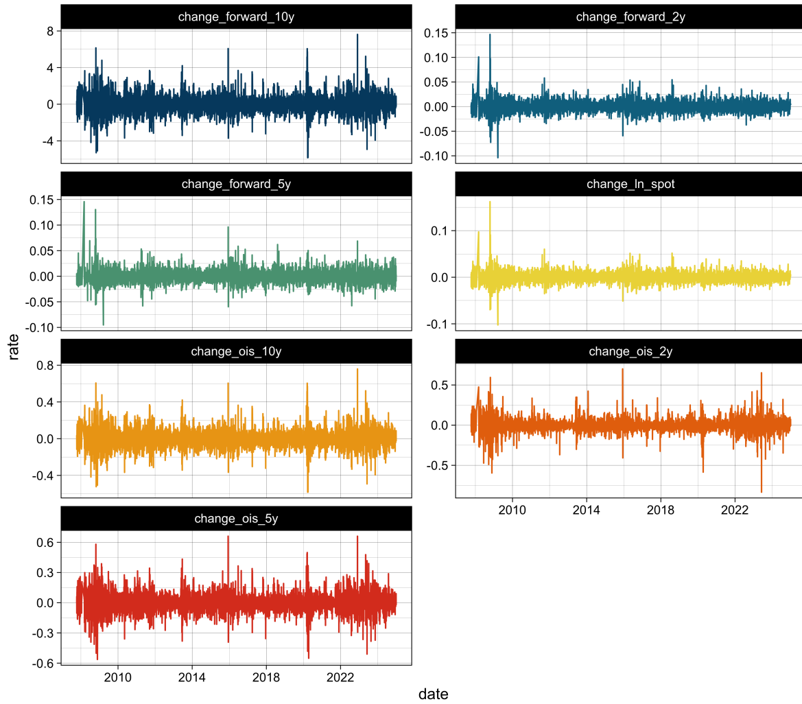
Figure A3: Key variables
