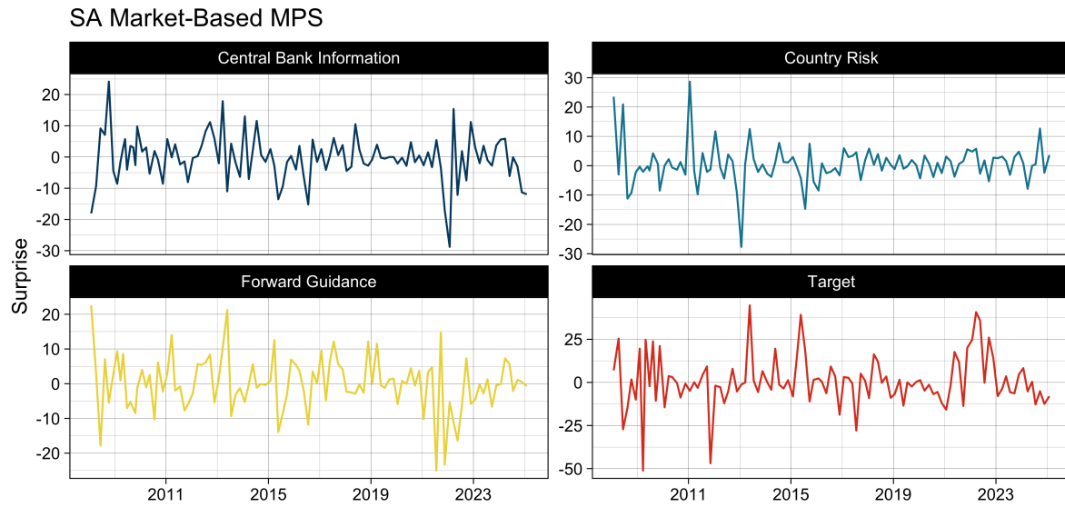
Figure A1: SA monetary policy surprises
