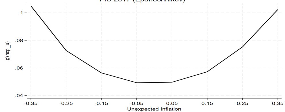
Pre-2017 (Epanechnikov)
