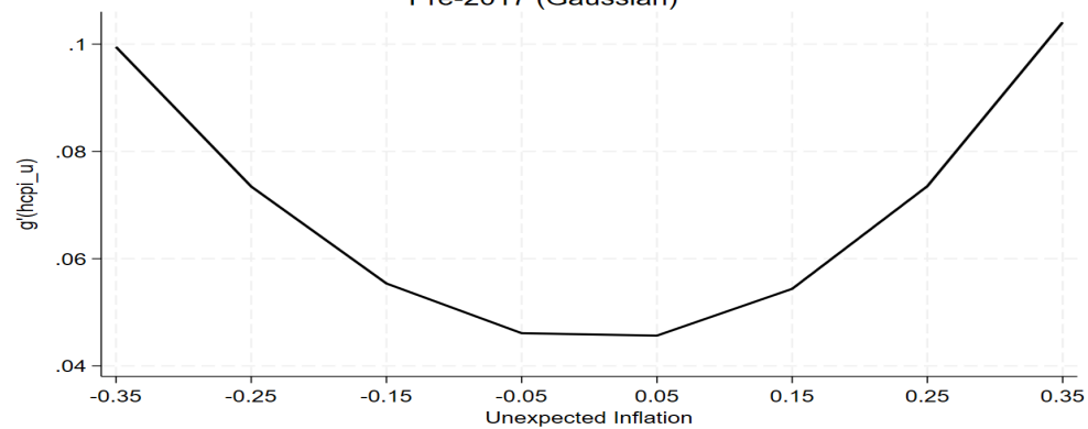
Pre-2017 (Gaussian)
