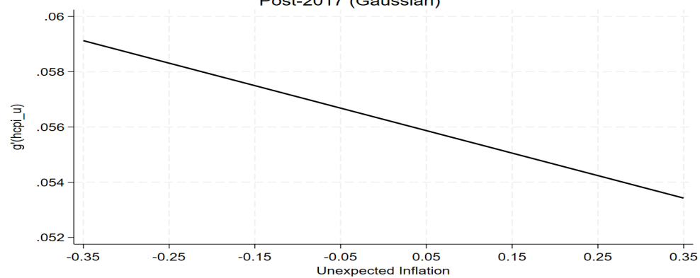
Post-2017 (Gaussian)
