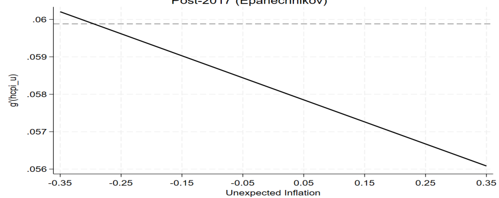
Post-2017 (Epanechnikov)
