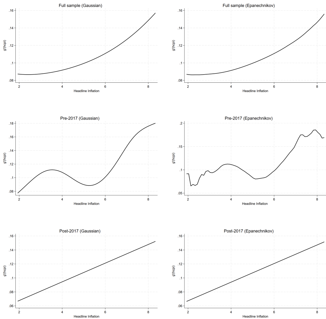
Figure 5: Semi-parametric regressions
