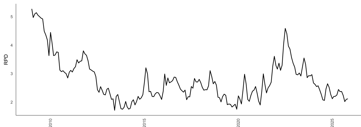
Figure 1: RPD over-time
