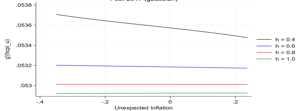
Robustness test: Bandwidth selection
