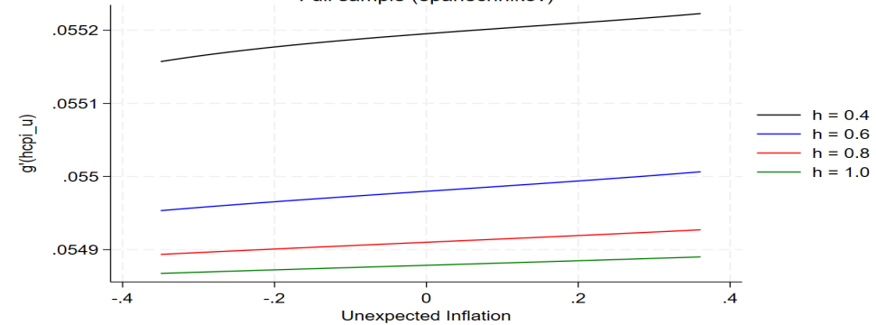
Robustness test: Bandwidth selection
