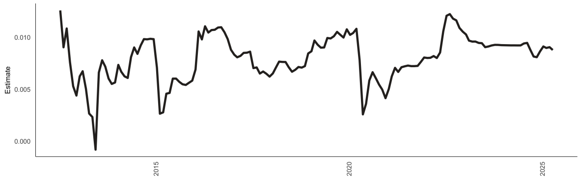
Figure 4: Recursive regression results of RPV on absolute inflation
