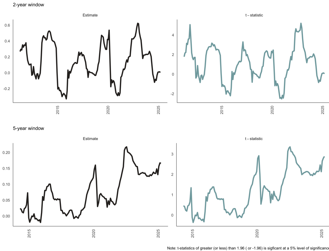
Figure 4: Rolling regression
