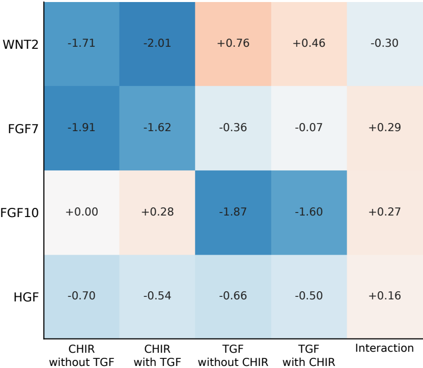
A Support genes
