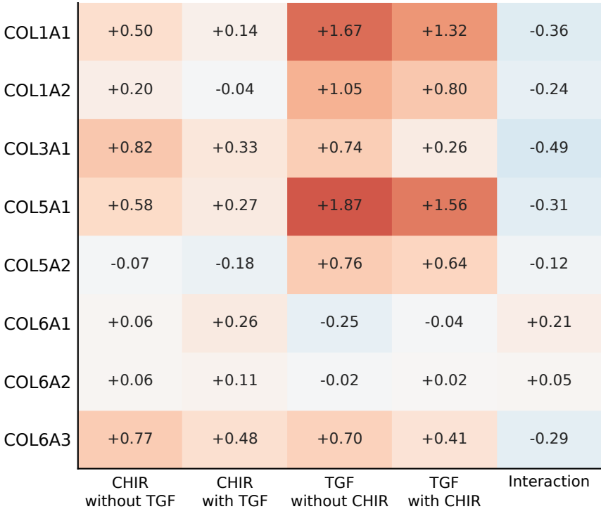
B Collagen genes
