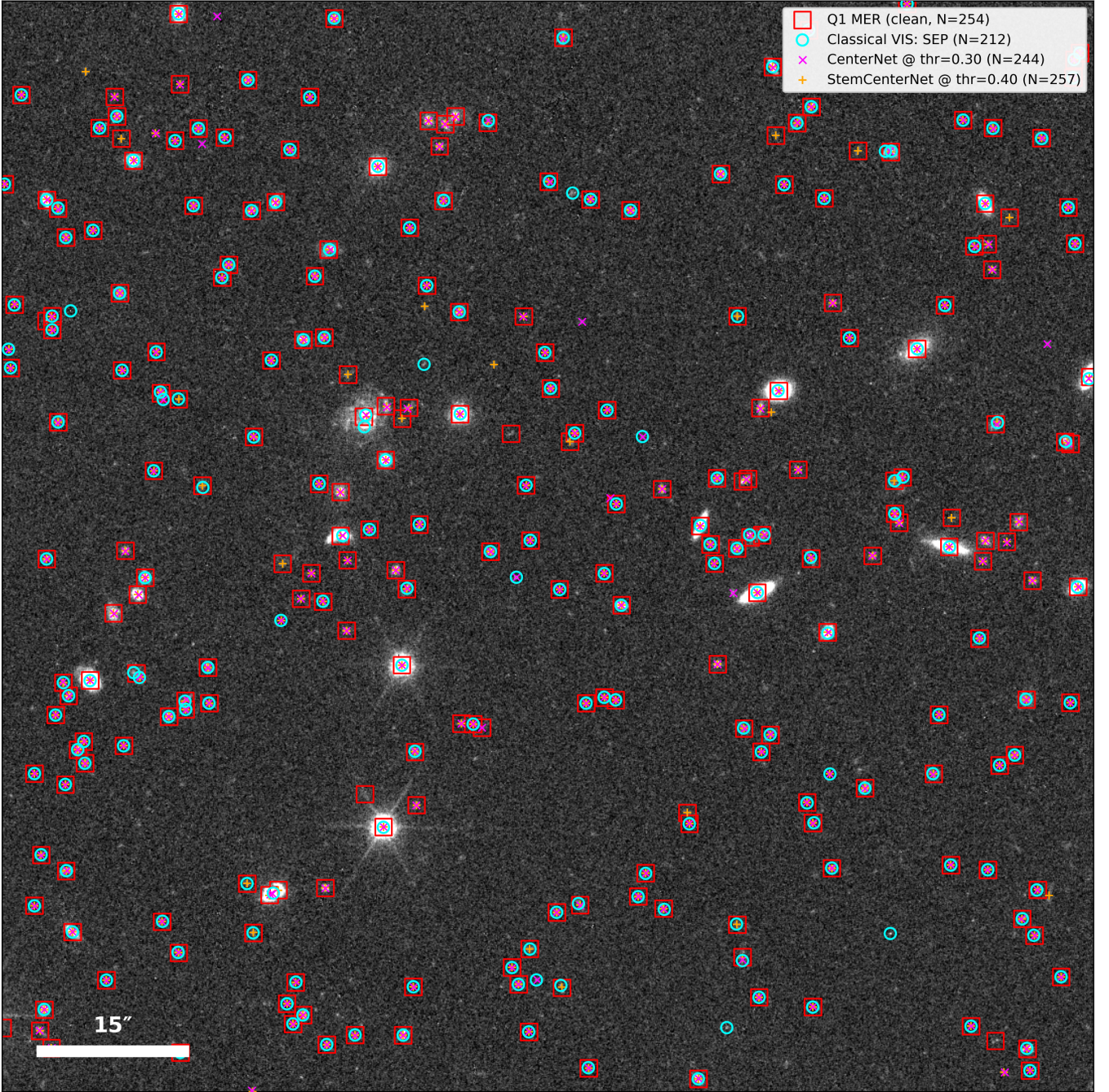
Figure 5. Detection on a single held-out Euclid VIS tile: the foundation head against classical and catalog references. A 1.7' tile (tile_x01792_y00000, 0.1'' \text{ px}^{-1} , from a spatially disjoint patch excluded from detection training), with four source lists overlaid. Cyan circles : the classical VIS source list (SEP extraction at 3\sigma , cleaned of diffraction-spike artifacts and duplicates). Magenta crosses : the foundation CenterNet head reading the frozen, fused ten-band bottleneck. Orange pluses : the StemCenterNet variant reading the native per-instrument stems. Red squares : the clean Euclid Q1 MER catalog (VIS-detected, non-spurious), drawn larger so that the square frames the circle where both lists agree. The legend gives each list's count on this tile; a source with a cross but no cyan circle is a head detection below the SEP 3\sigma baseline, the depth gain quantified in Figure 6. The white bar is 15'' .
