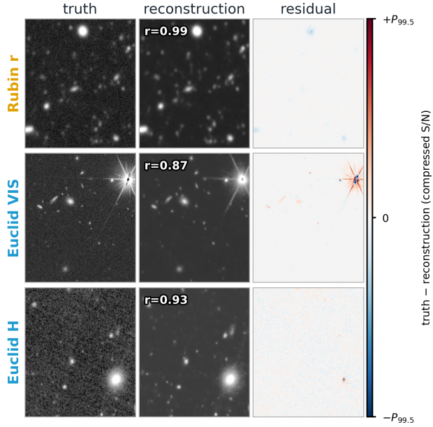
Figure 3. Masked-band reconstruction on three held-out ECDFS tiles. In each row a single band is withheld and reconstructed from the other nine: Rubin r (top), Euclid VIS (middle), and Euclid NISP H (bottom). Columns show the true band (left), the reconstruction (center), and the residual truth – reconstruction (right); panels are 48'' on a side. Images use compressed S/N units, with residual limits \pm P_{99.5} of each truth crop. After undoing the compression, the maximum absolute residuals are 45.8, 177.1, and 10.6 times the local input pixel RMS for Rubin r , VIS, and H , respectively; these extremes occur in the cores of the brightest point sources, where the compressed display saturates, and residuals elsewhere are far smaller. The annotated r is the Pearson correlation between truth and reconstruction over the brightest 10% of pixels; averaged across the 39 held-out tiles the mean per-band correlation is 0.99 ( r ), 0.77 (VIS), and 0.90 ( H ).
