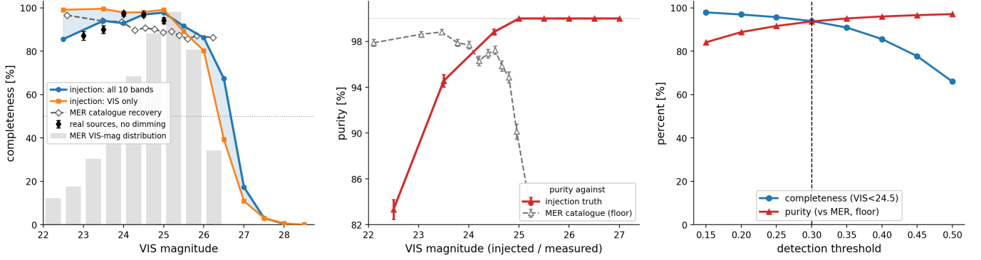
Figure 6. Detection performance of the fused CenterNet head evaluated within the 108 patch-25 tiles excluded from head training. Point-source completeness uses the 45 tiles with sufficient local donors; the injection-purity test uses all 108 tiles. Left: completeness versus VIS magnitude from source-recycling injection: real unresolved donors, carrying their full ten-band cutouts, dimmed to each target magnitude and placed in all ten bands (blue) or in VIS only (orange); the shaded band is the \approx 0.3 mag fusion gain, giving a 50% point-source depth of \text{VIS} \approx 26.7 . Black diamonds are real sources re-injected at native brightness, validating the dimming; their bright-end dip, shared with the all-band curve while in-situ MER recovery holds at \sim 97\% , is an artifact of the copied stamps, not of the detector on real sky. The dashed curve is in-situ recovery of the clean VIS-selected Q1 MER sample and the gray histogram its VIS-magnitude distribution; a near-zero-flux control bounds the protocol’s chance floor below 0.66% (95% CL). Center: P_{\text{inj}} (Equation 3; filled), 100% at the sampled magnitudes 25–27 with the bright-end decline from bright-star wing detections, and catalog-based purity against the full MER catalog (open), whose faint-end drop tracks the MER turnover. The two statistics use different denominators. Right: completeness ( \text{VIS} < 24.5 ) and catalog-based purity versus detection threshold; the dashed line marks the 0.30 working point.
