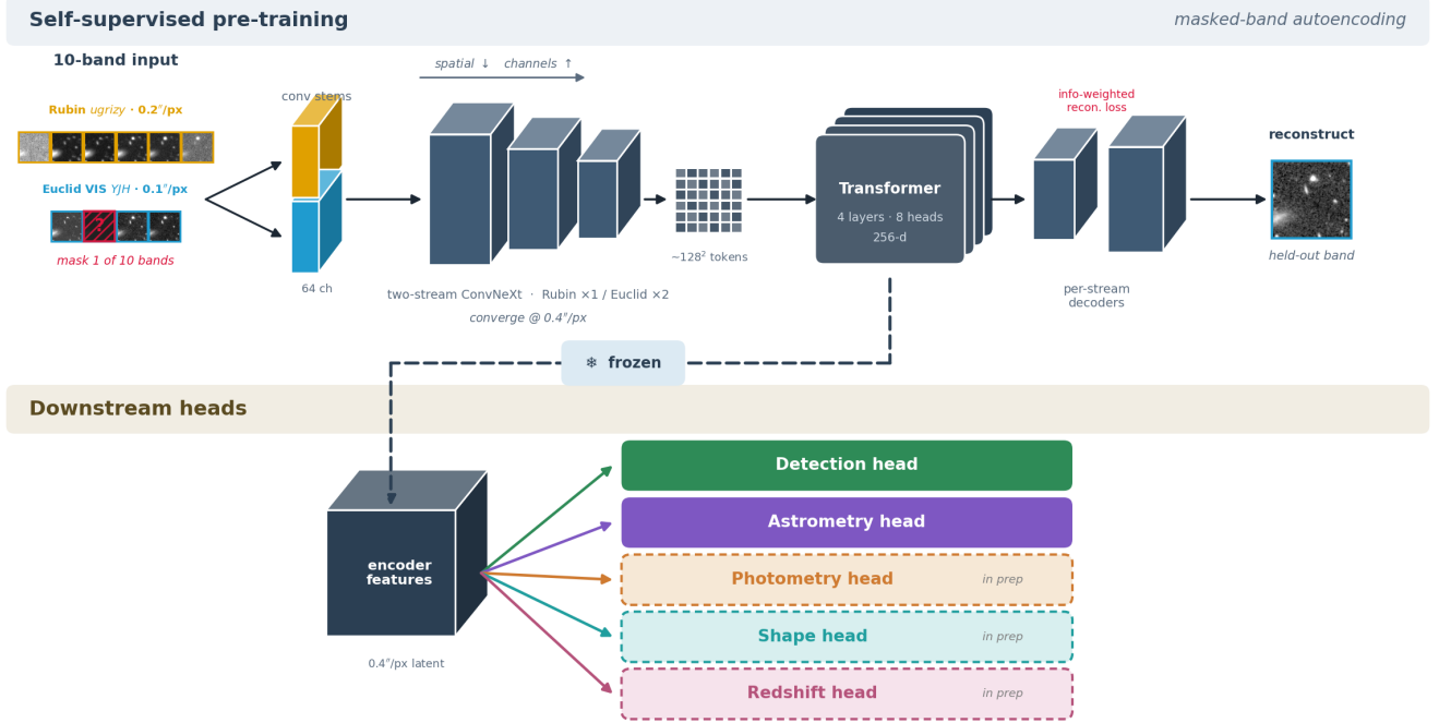
Figure 2. Model architecture. Top: self-supervised pretraining by masked-band autoencoding. The ten input bands, Rubin ugrizy at 0.2'' \text{ px}^{-1} and Euclid VISYJH at 0.1'' \text{ px}^{-1} , pass through per-band convolutional stems and a two-stream ConvNeXt encoder (Rubin and Euclid branches) whose feature maps shrink spatially and deepen in channels until they converge on a common 0.4'' \text{ px}^{-1} grid. A transformer bottleneck (4 layers, 8 heads, 256-d) mixes the \sim 128^2 fused tokens, each carrying joint Rubin–Euclid features for one 0.4'' \text{ px}^{-1} location, and per-stream decoders reconstruct the single held-out band under an information-weighted loss; the complete model totals \sim 9.1\text{M} parameters. Bottom: for downstream tasks the encoder is frozen and its 0.4'' \text{ px}^{-1} latent features feed lightweight task heads, detection and astrometry in this work, with photometry, shape, and redshift heads in preparation. Input and reconstruction thumbnails show the same matched ECDFS tile as Figure 1.
