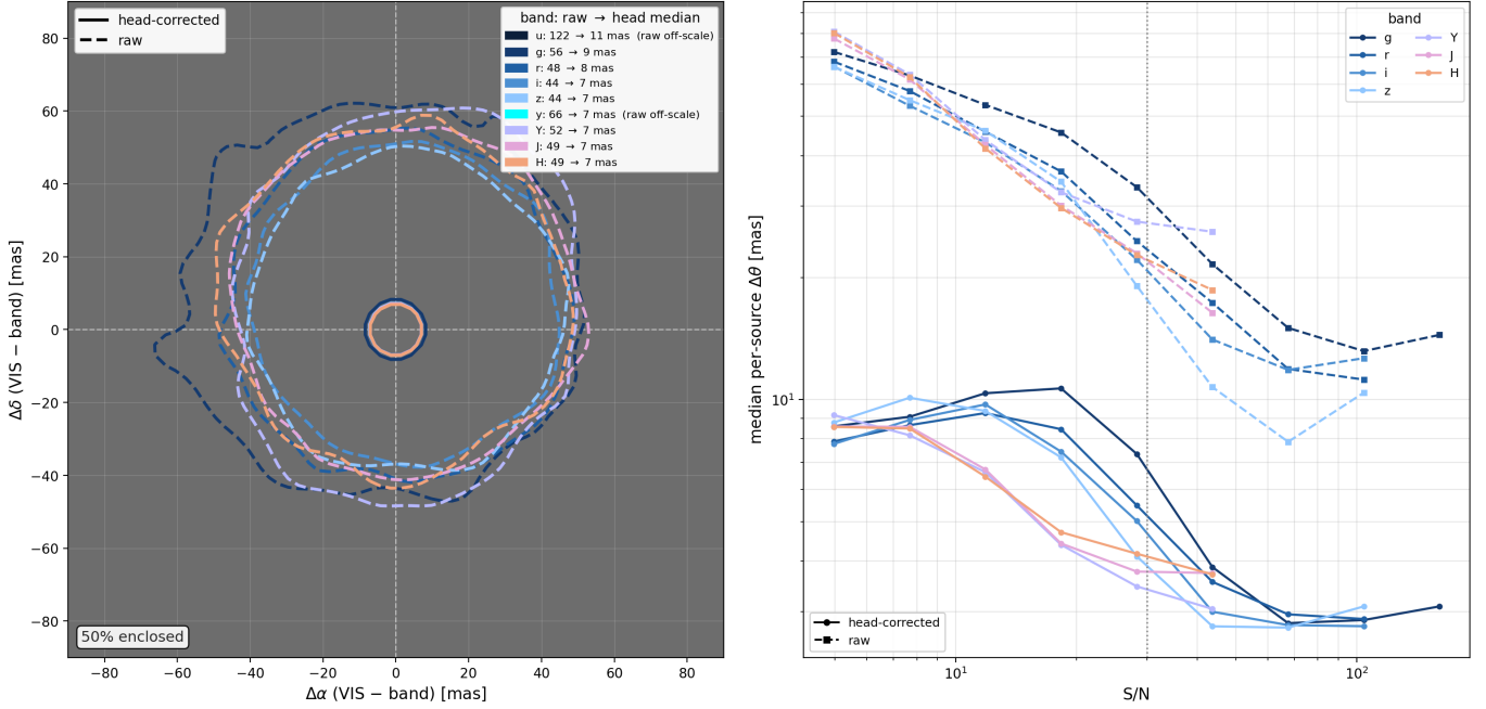
Figure 8. Effect of the per-source position head on cross-survey agreement, using the same offset measurement as Figure 7 ( Euclid VIS – Rubin/NISP; Equation 1) over all 790 ECDFS tiles. Solid curves are head-corrected positions; dashed curves are the raw classical centroids. Left: all-detection offset clouds, each contour enclosing 50% of that band’s sources. The head collapses the raw \sim 50 mas clouds to \sim 6 – 10 mas and re-centers them on the origin, removing both the per-source scatter and the systematic offset; the legend gives the raw \rightarrow head median per band ( u and y raw clouds lie off the plotted scale). Right: median per-source radial offset versus S/N: the head-corrected curves (solid) are far flatter than the raw (dashed), staying near the bright-source floor across the full range, with the in-model centroid anchor holding the bright end at the classical systematics floor. These medians measure agreement with the VIS-centroid convention that also supplies the head’s training labels, so they can sit below the accuracy against truth, which is bounded by the VIS anchor and measured directly in Figure 9.
