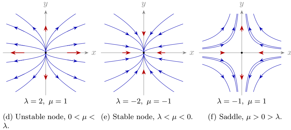
Figure 1.14: Phase portraits of \dot{x} = \lambda x , \dot{y} = \mu y . Blue curves are y = y_0 (x/x_0)^{\mu/\lambda} ; red half-lines are the trajectories on the coordinate axes. Arrows indicate the direction of increasing time.
