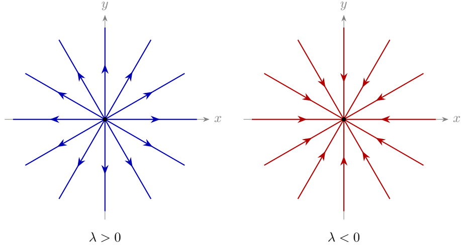
Figure 1.13: Phase portrait for A = \lambda I . The trajectories are escaping from the origin ( \lambda > 0 ) or attracted by the origin ( \lambda < 0 ).
