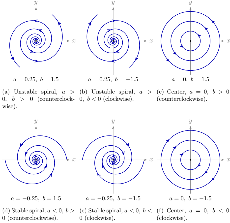
Figure 1.15: Phase portraits of \dot{z} = Bz with e^{tB} = e^{at}R_{bt} . The sign of a determines whether trajectories move away from ( a > 0 ) or towards ( a < 0 ) the origin, while the sign of b determines the sense of rotation. Arrows indicate the direction of increasing time.
